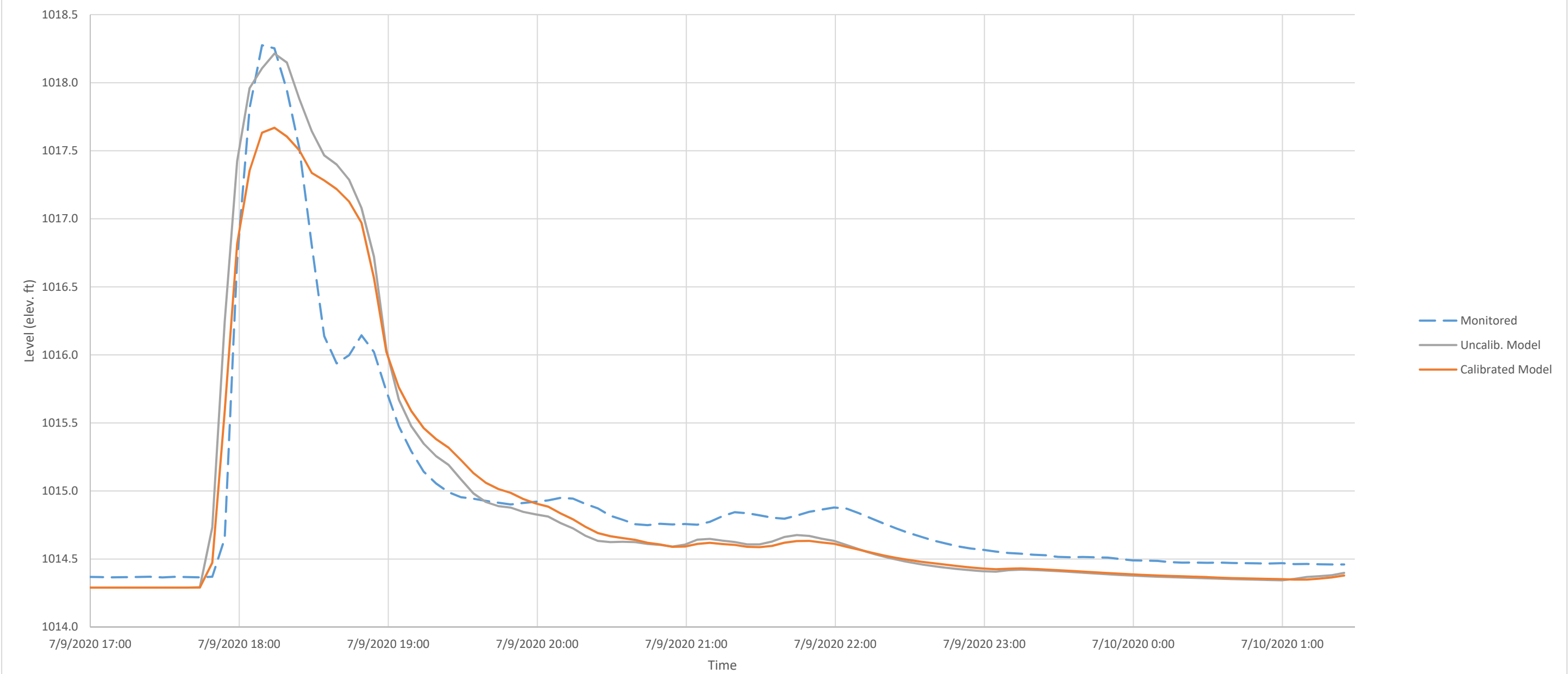
Riva Rd. Level Logger - July 9
