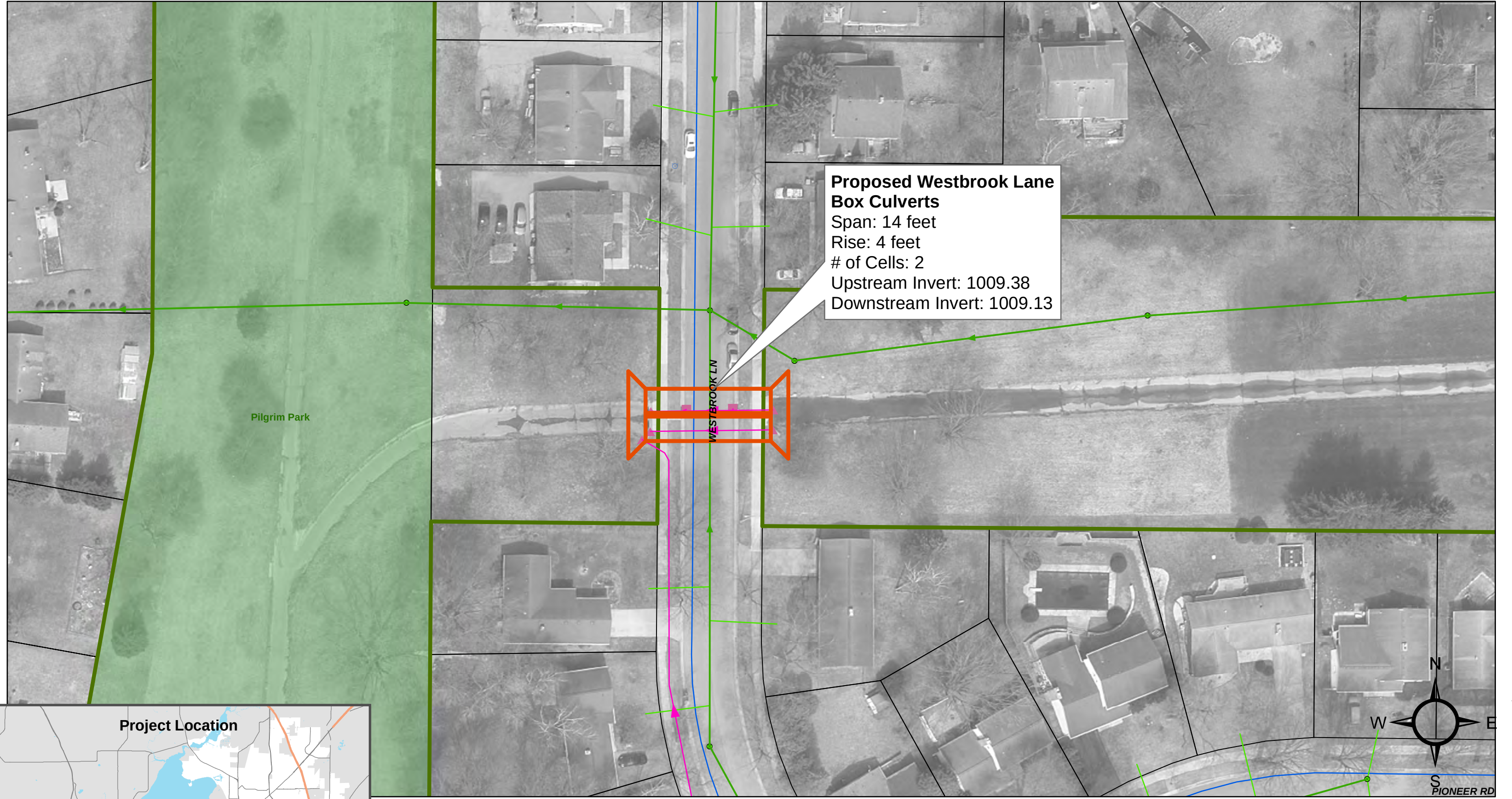
Figure 9-13 Westbrook Lane Box Culverts East Badger Mill Creek Watershed
