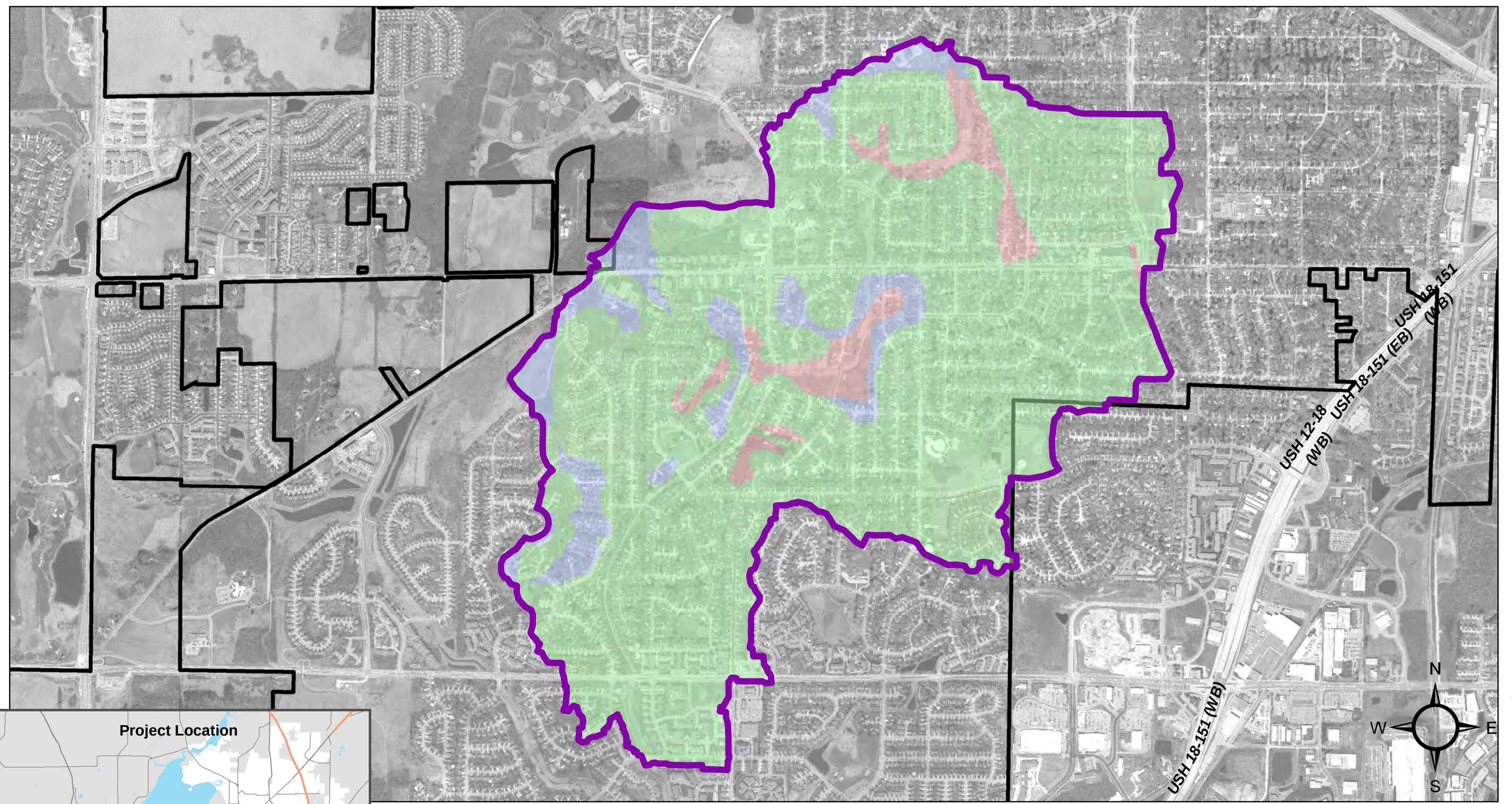
Figure 2-3 Hydrologic Soil Groups East Badger Mill Creek Watershed
