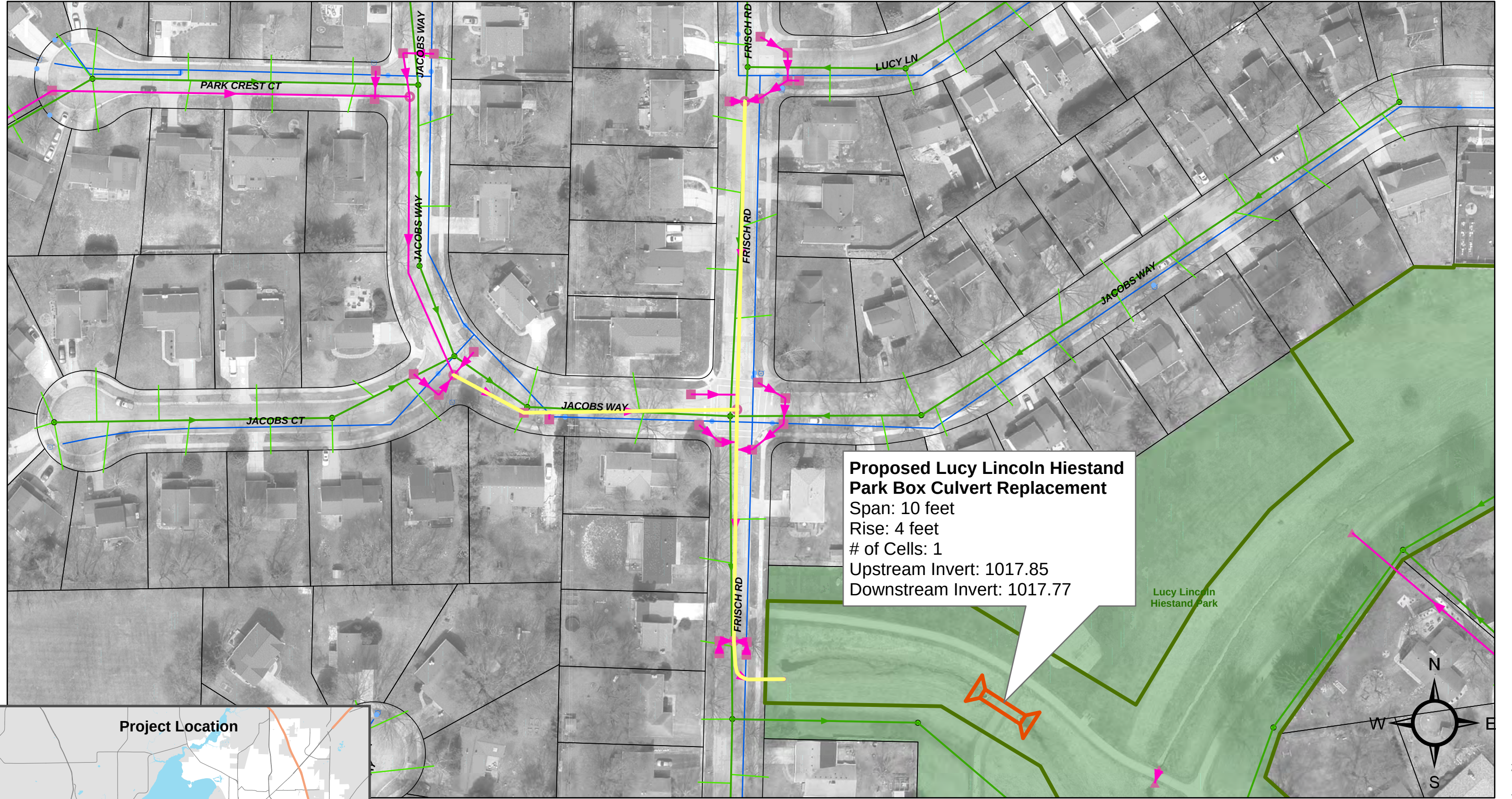
Figure 9-14 Lucy Lincoln Hiestand Park Culvert and Frisch Road Storm Sewer East Badger Mill Creek Watershed
