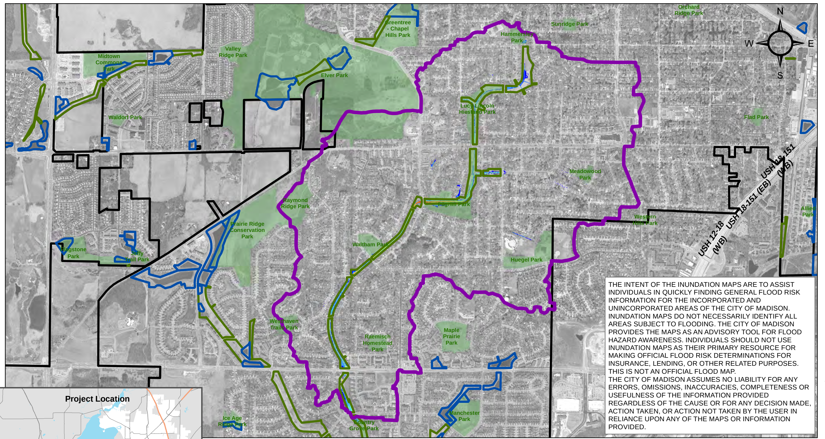
Figure 6-1 Existing Conditions Inundation Mapping 100% Chance Event East Badger Mill Creek Watershed
