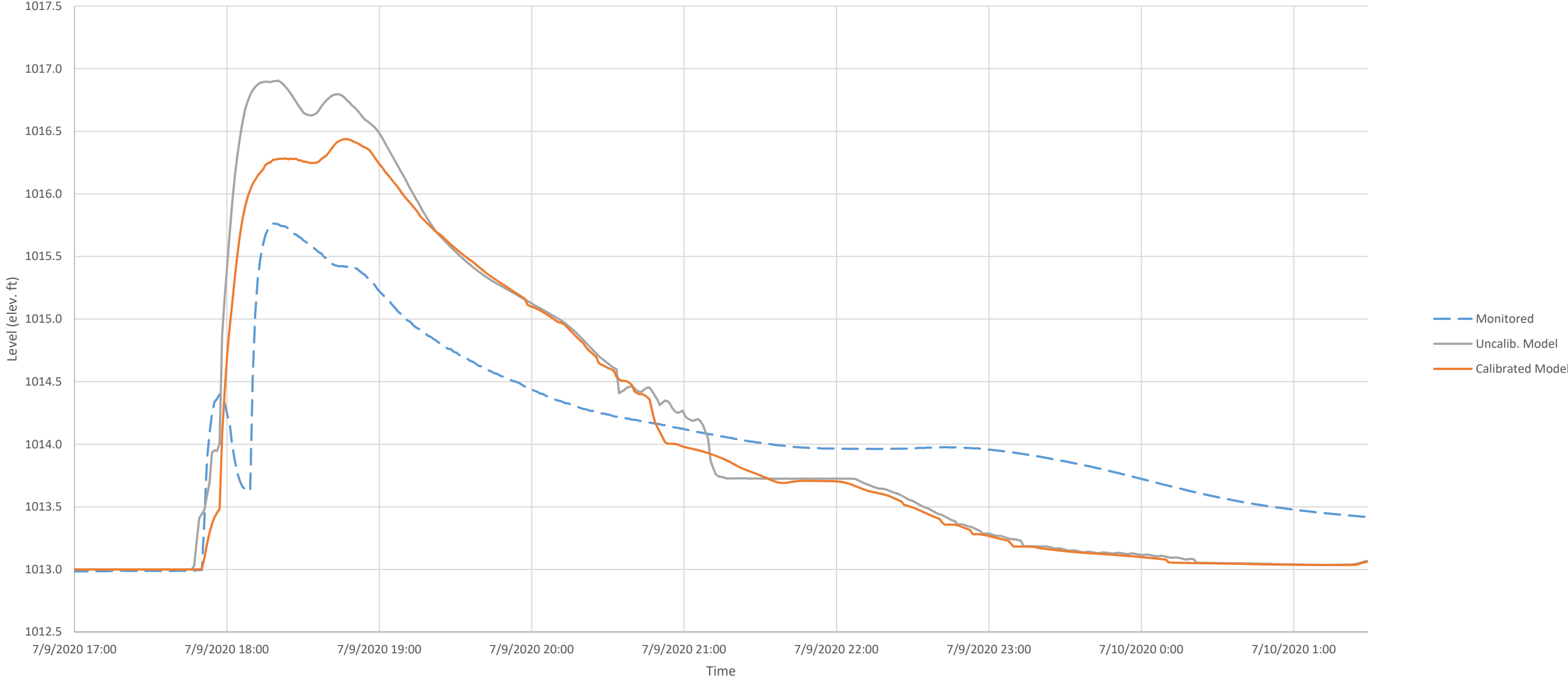
Raymond Rd. Level Logger - July 9
