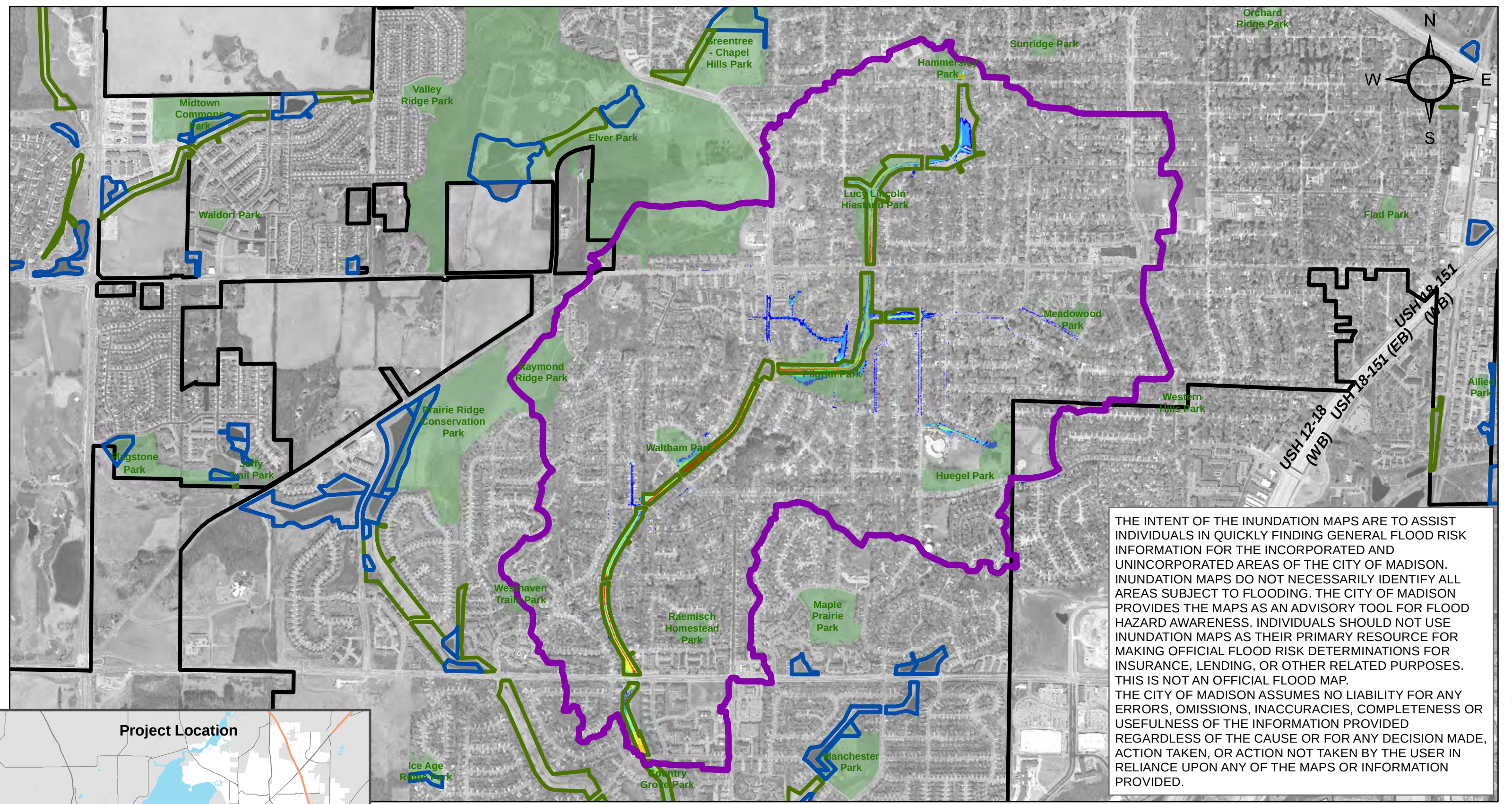
Figure 10-5 Proposed Conditions Inundation Mapping 4% Chance Event East Badger Mill Creek Watershed
