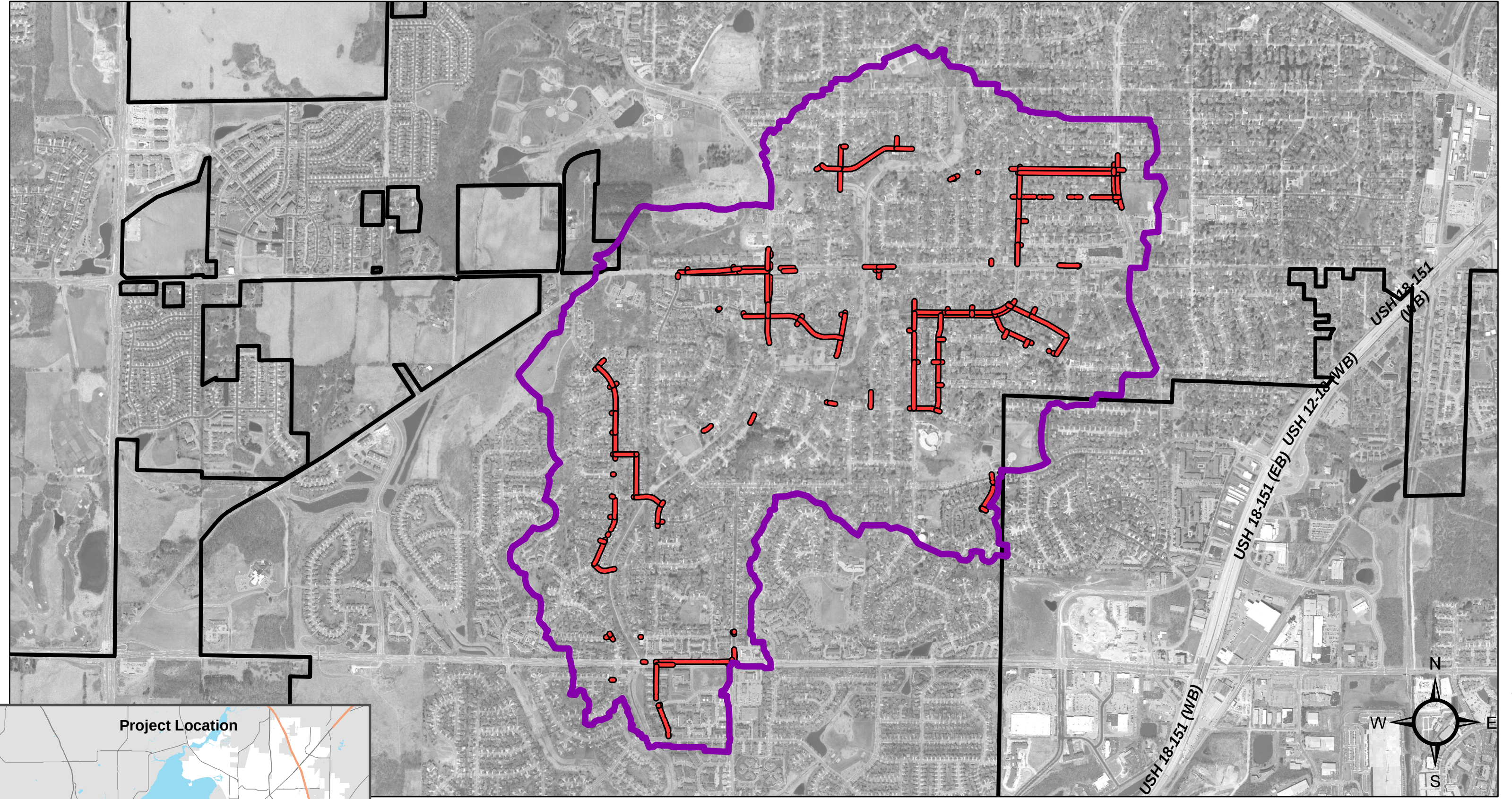
Figure 6-11 Existing Conditions Streets Not Meeting 10% Chance Event Target East Badger Mill Creek Watershed
