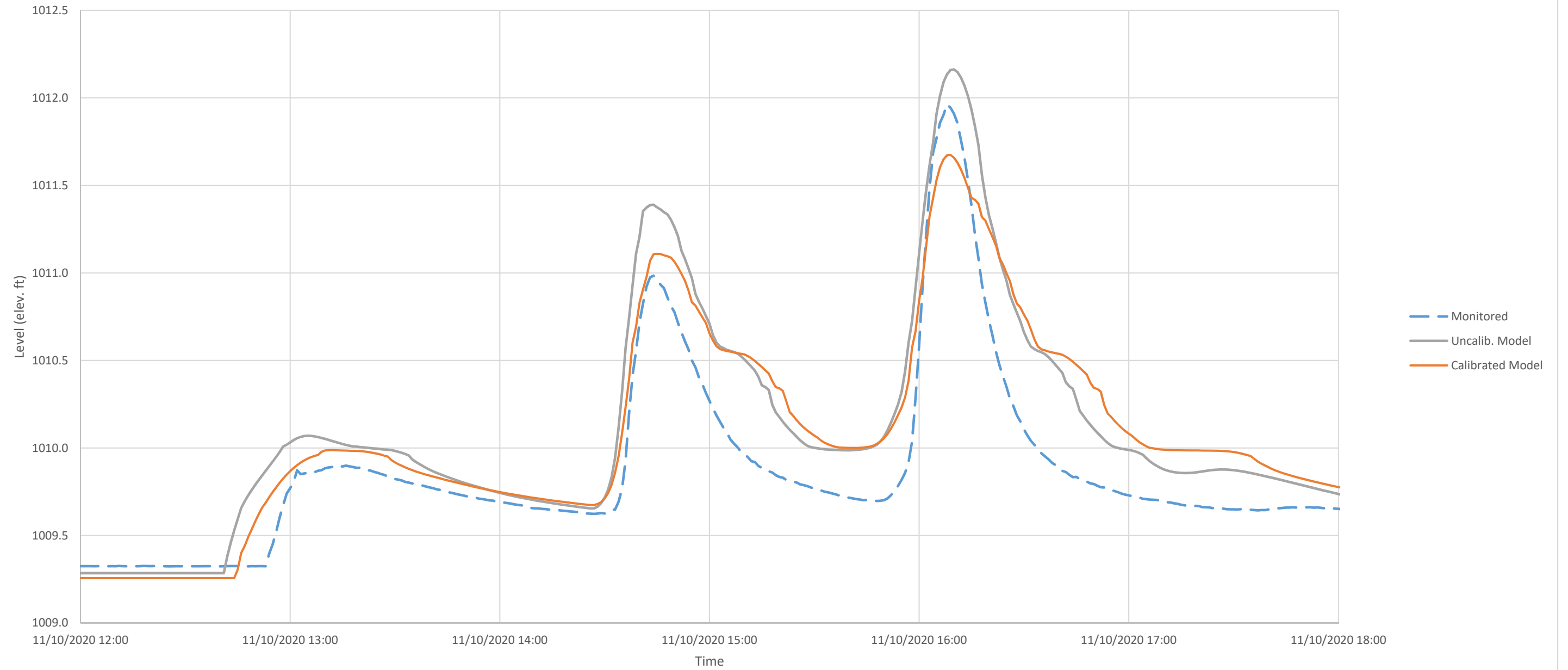
Westbrook Ln. Level Logger - November 10
