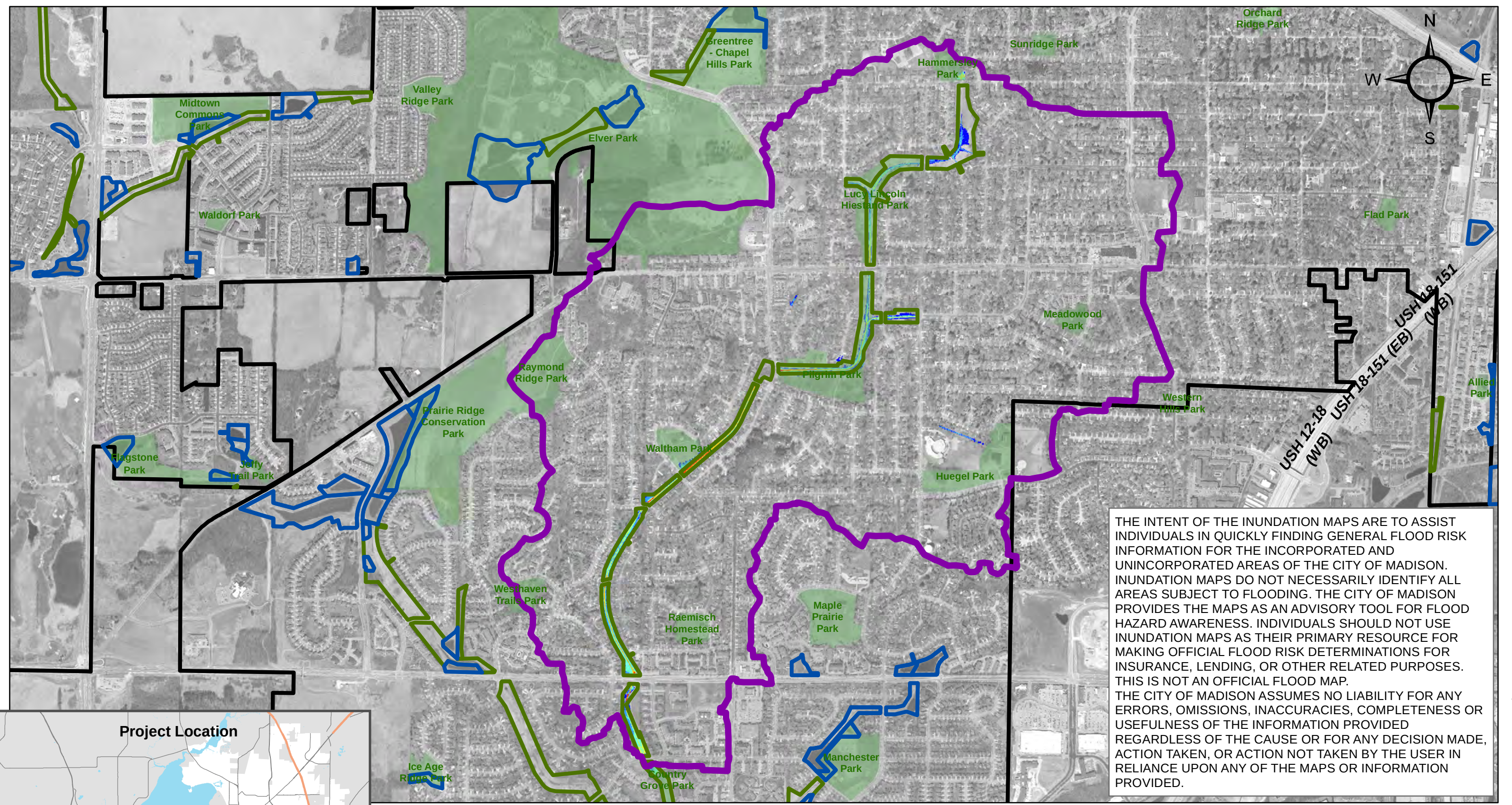
Figure 10-3 Proposed Conditions Inundation Mapping 20% Chance Event East Badger Mill Creek Watershed
