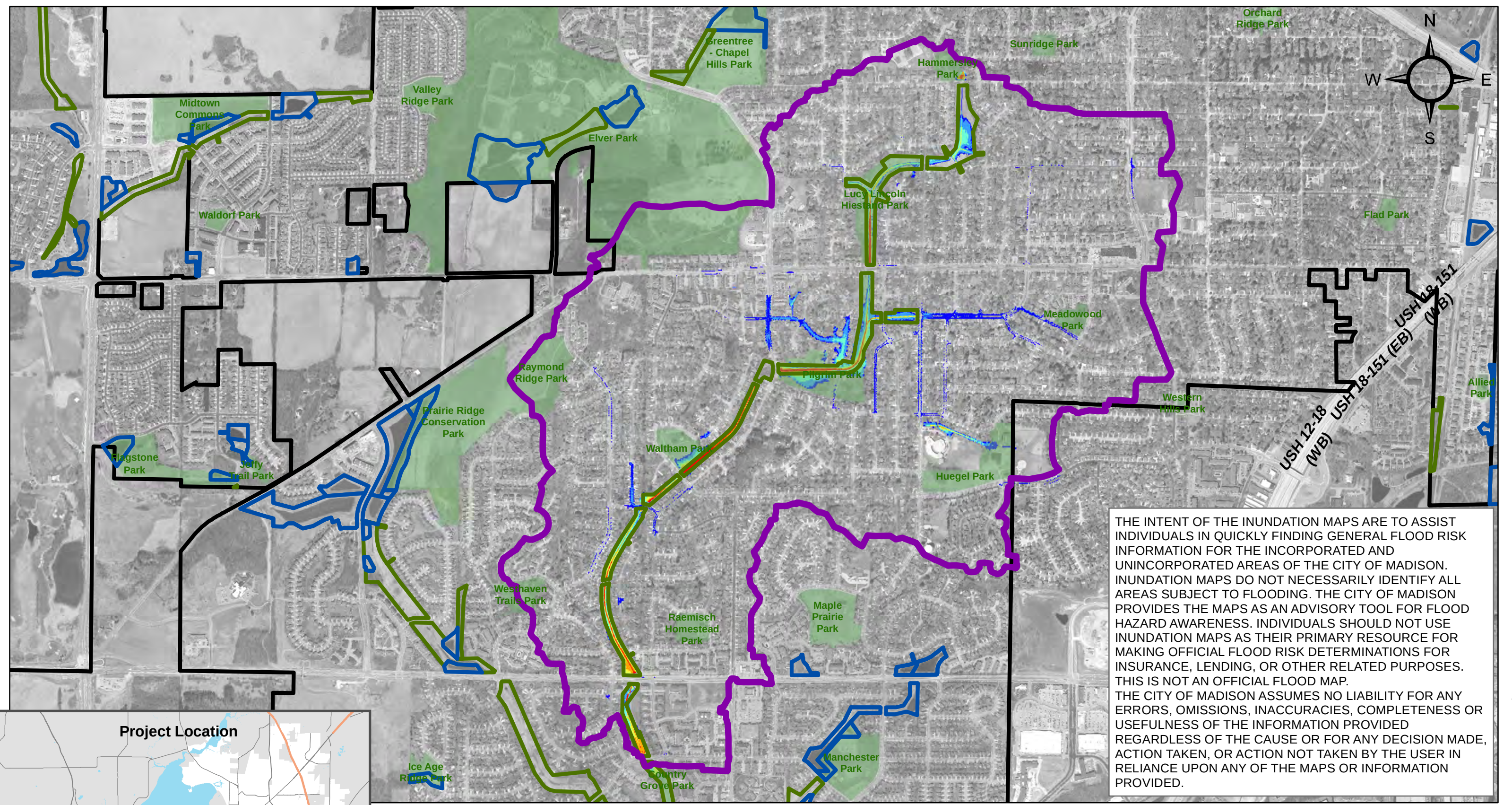
Figure 10-6 Proposed Conditions Inundation Mapping 2% Chance Event East Badger Mill Creek Watershed
