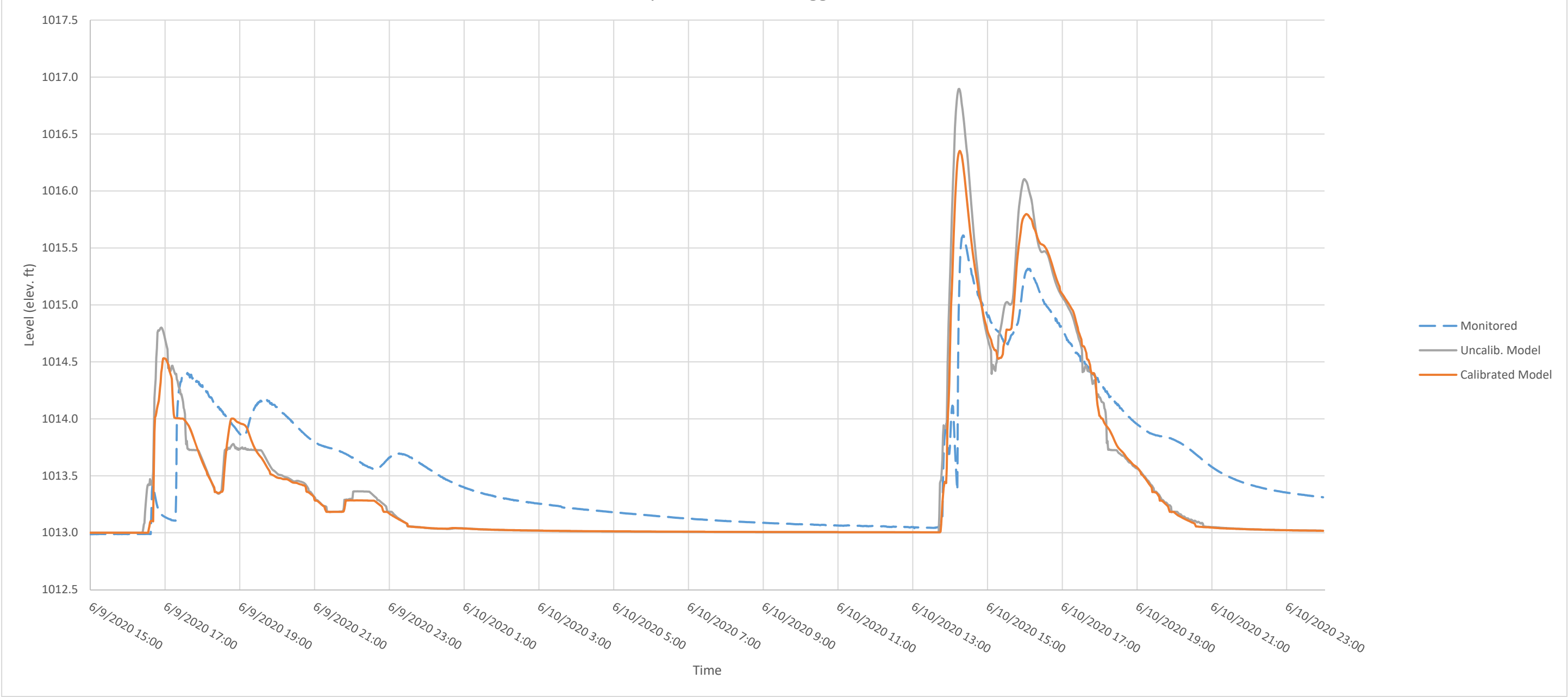
Raymond Rd. Level Logger - June 9-10
