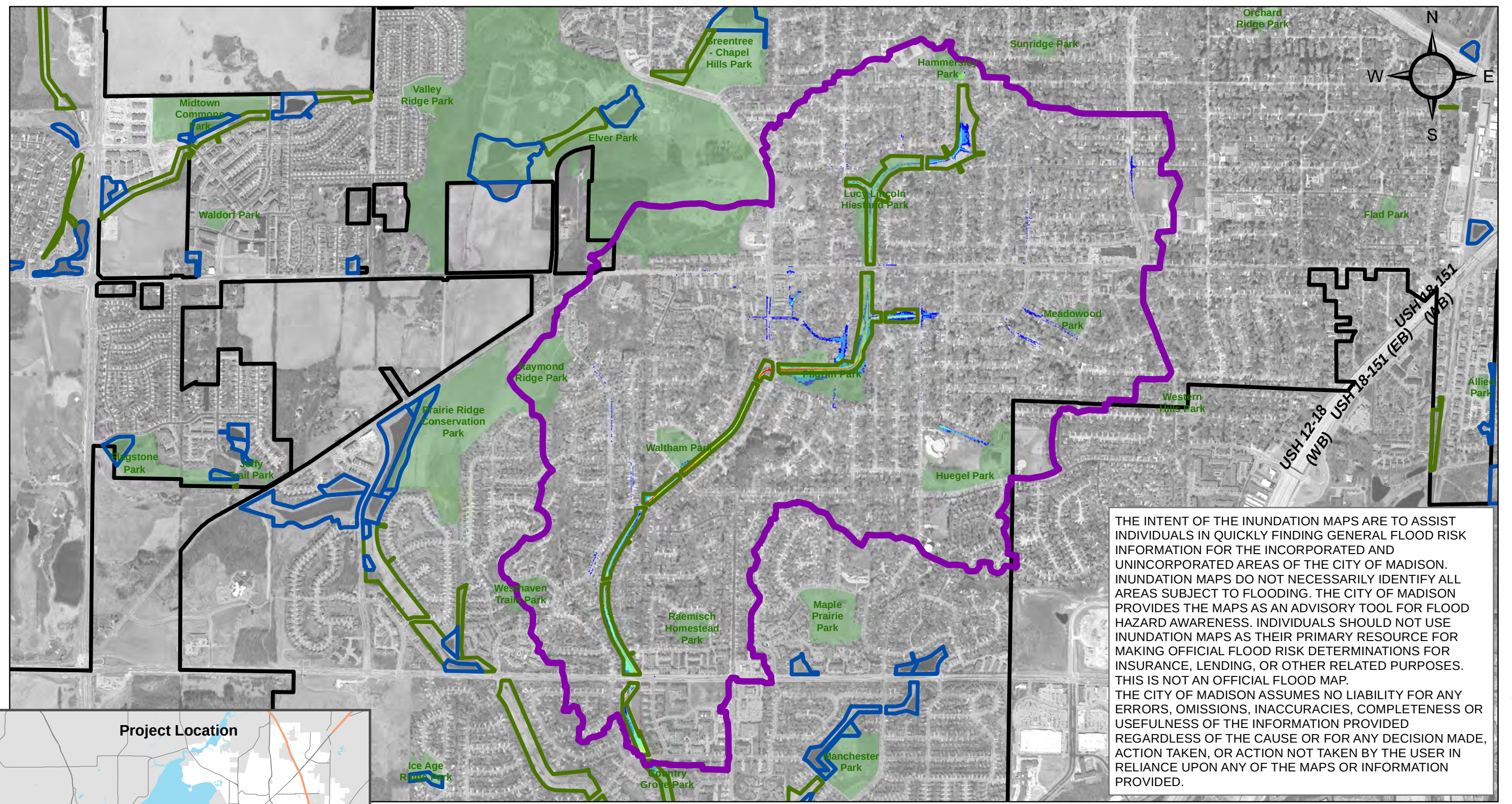
Figure 6-3 Existing Conditions Inundation Mapping 20% Chance Event East Badger Mill Creek Watershed
