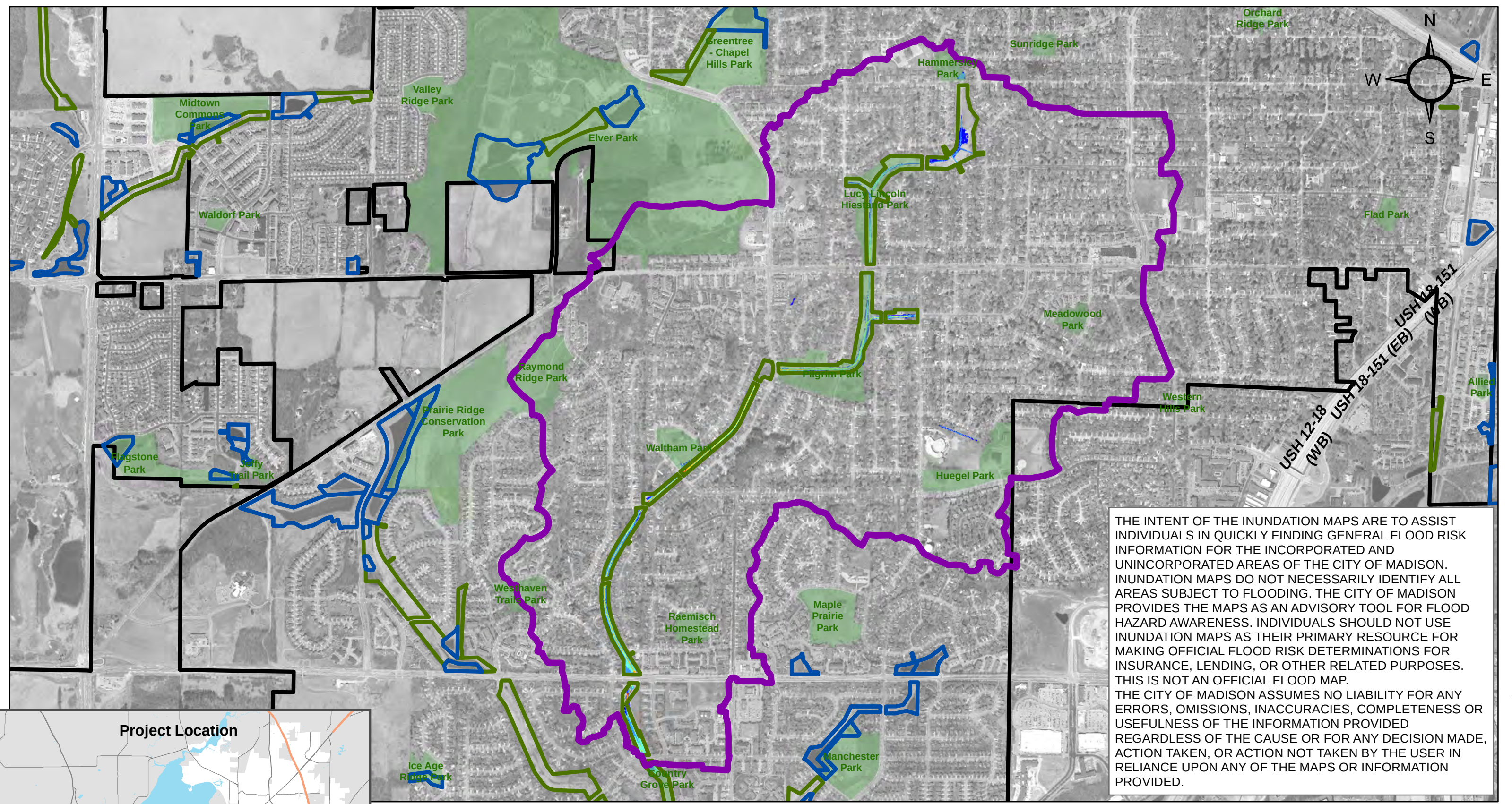
Figure 10-2 Proposed Conditions Inundation Mapping 50% Chance Event East Badger Mill Creek Watershed
