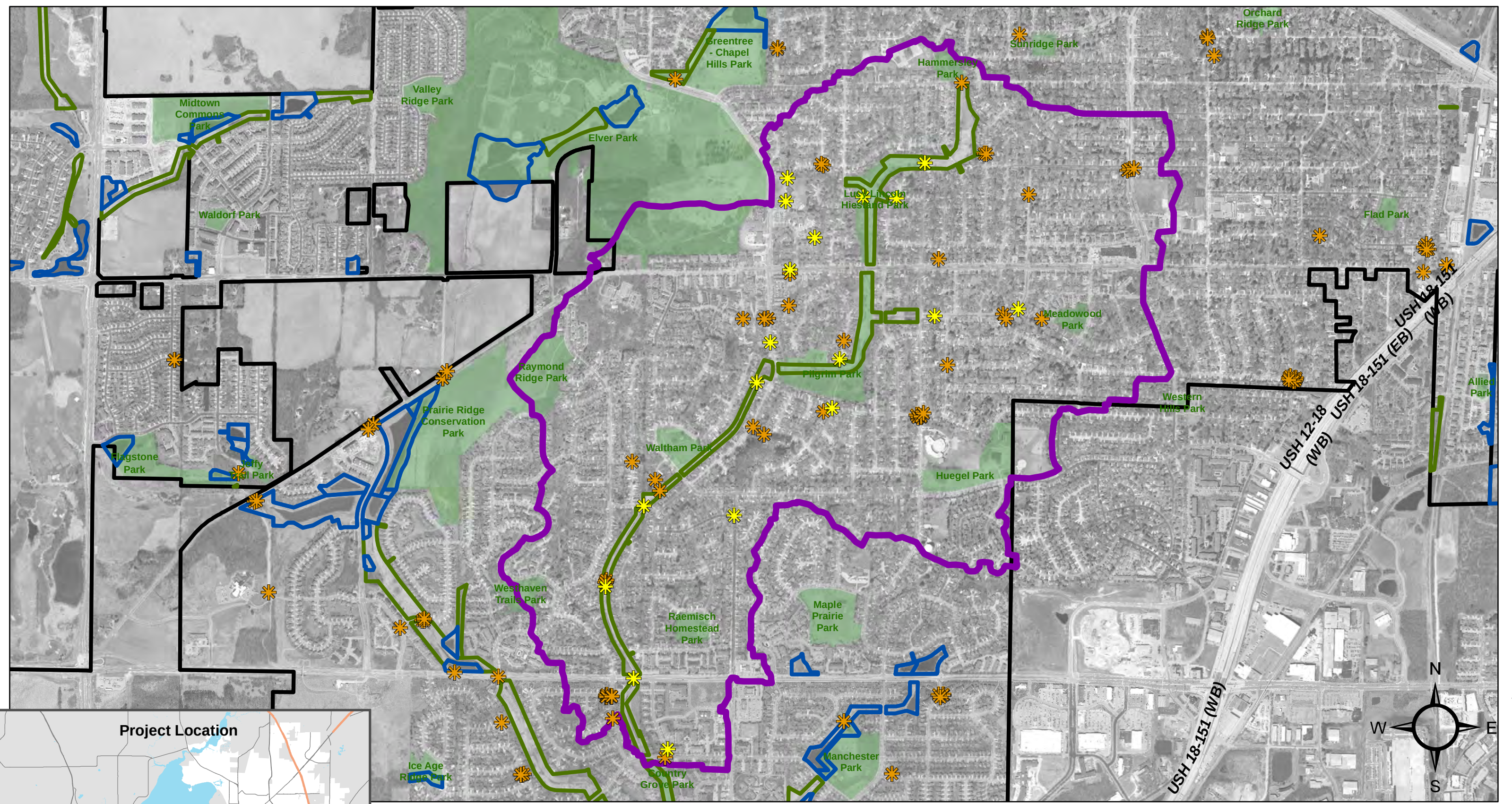
Figure 1-4 Flood Locations Reported by City Staff East Badger Mill Creek Watershed
