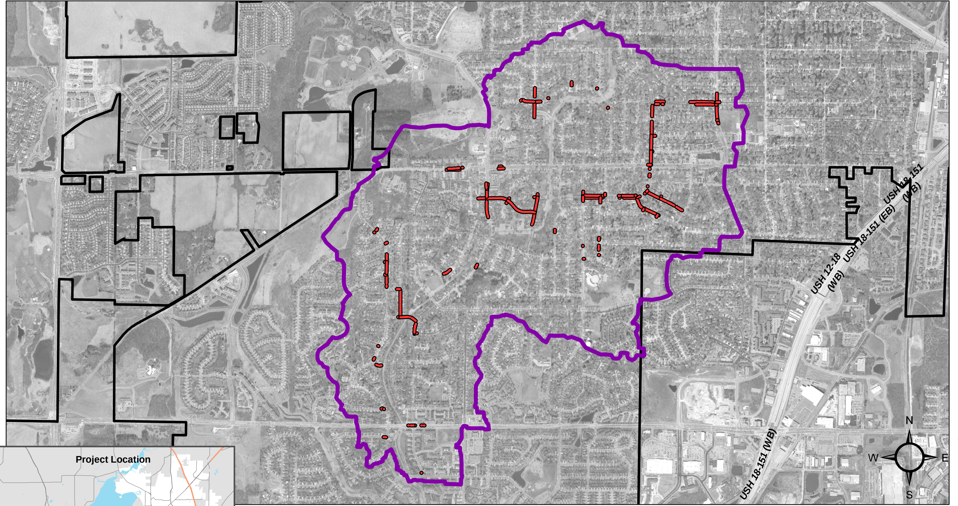
Figure 6-12 Existing Conditions Streets Not Meeting 4% Chance Event Target East Badger Mill Creek Watershed
