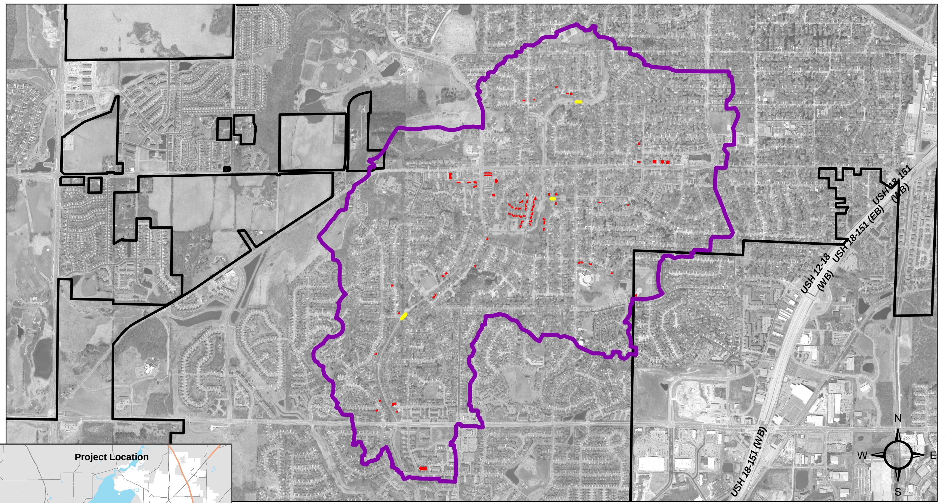
Figure 6-13 Existing Conditions Structures & Greenway Crossings Not Meeting 1% Chance Event Target East Badger Mill Creek Watershed
