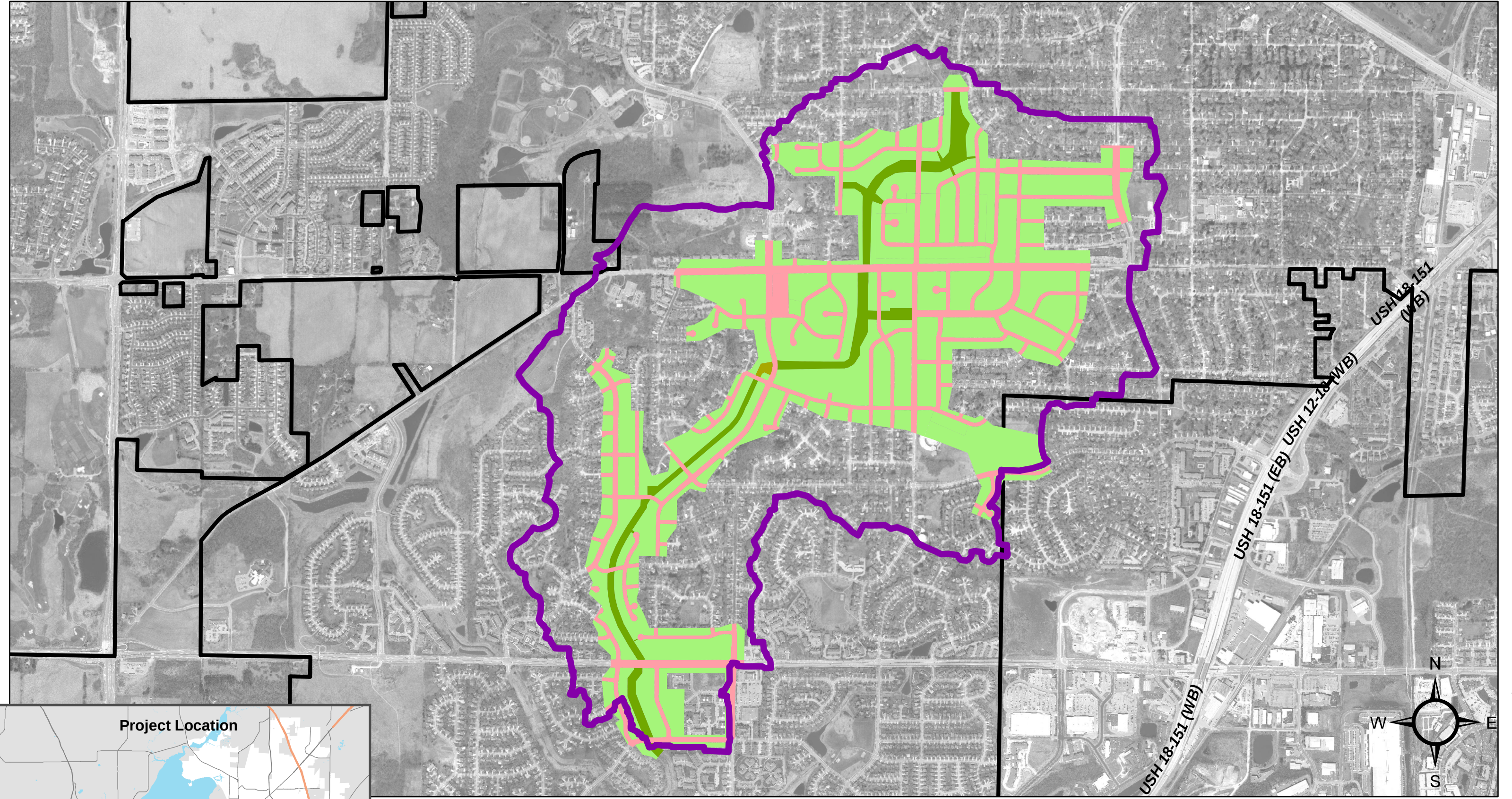
Figure 4-4 2D Model Roughness East Badger Mill Creek Watershed
