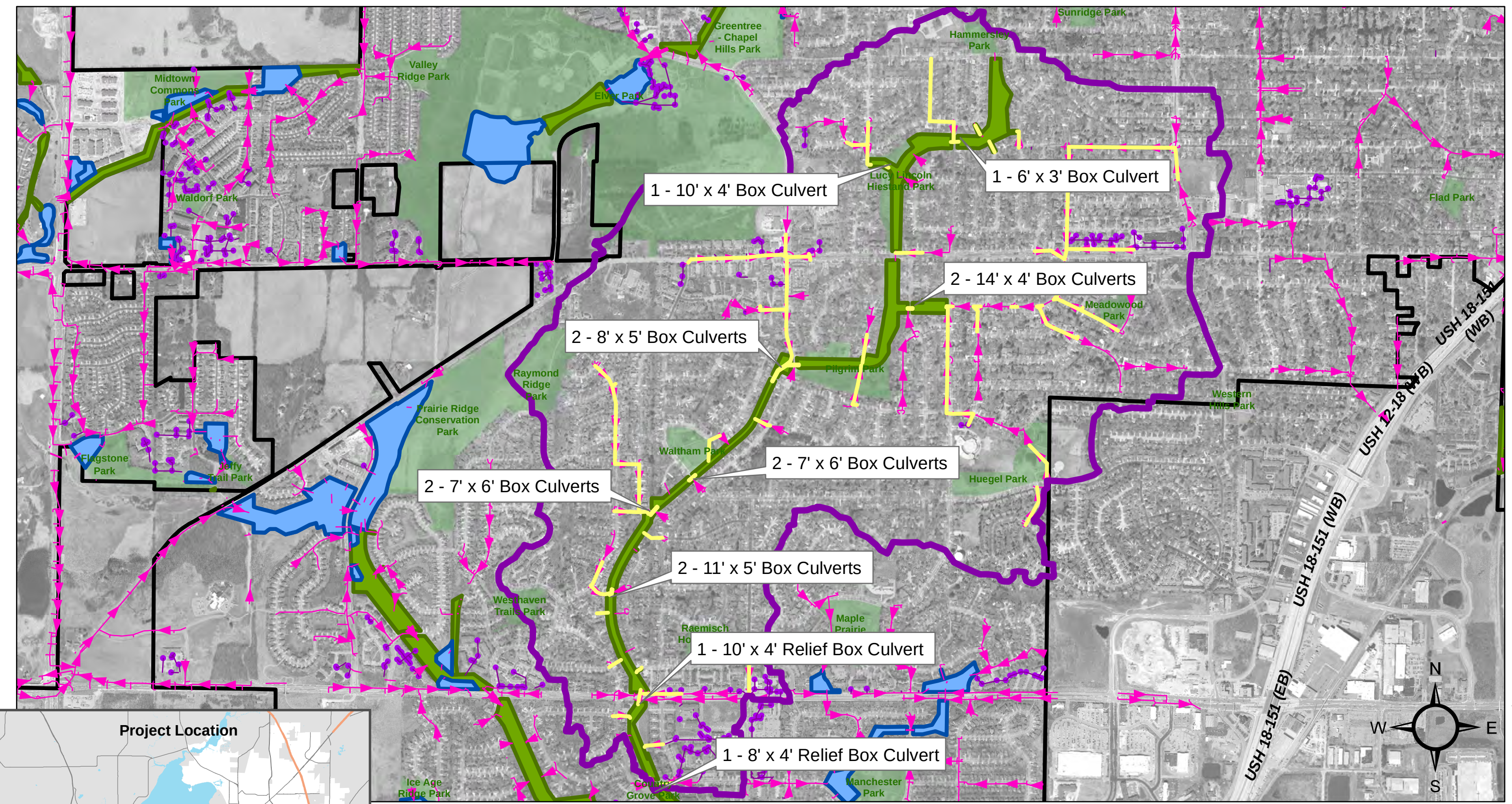
Figure 9-6 Greenway Crossing Improvement Overview East Badger Mill Creek Watershed
