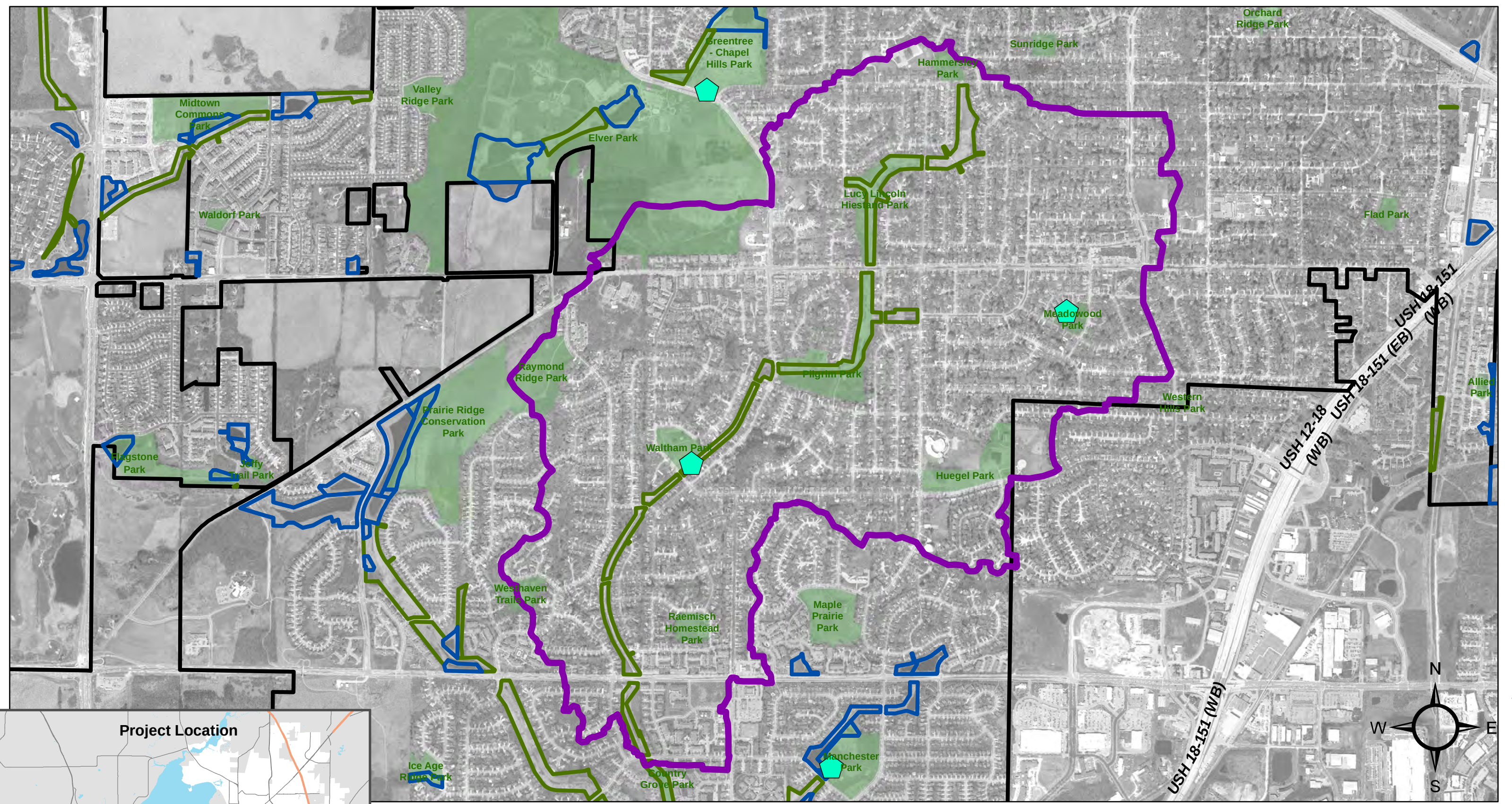
Figure 4-1 Rain Gage Locations East Badger Mill Creek Watershed
