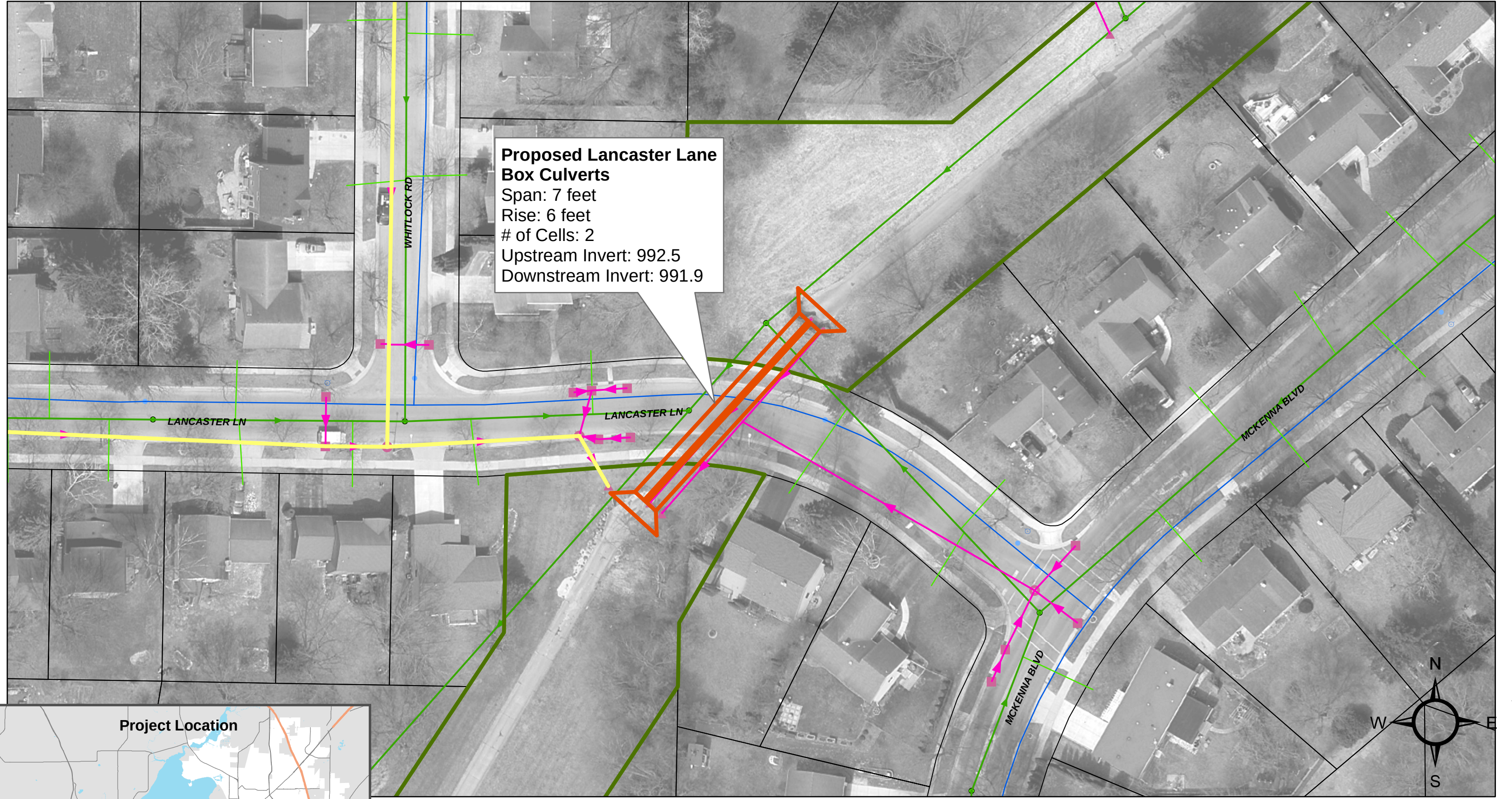
Figure 9-10 Lancaster Lane Box Culverts East Badger Mill Creek Watershed
