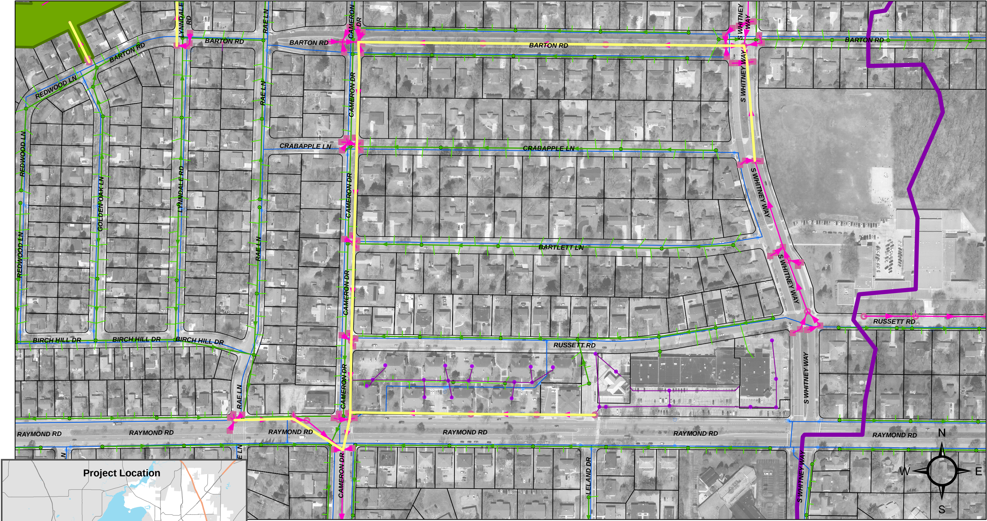
Figure 9-5 Raymond Road-Cameron Drive-Barton Road-Whitney Way Reconstruction East Badger Mill Creek Watershed 0 237.5 475 Feet N W E S *SEE REPORT FOR ADDITIONAL NOTES THAT IMPACT PROJECT IMPLEMENTATION Date: 2/3/2023
