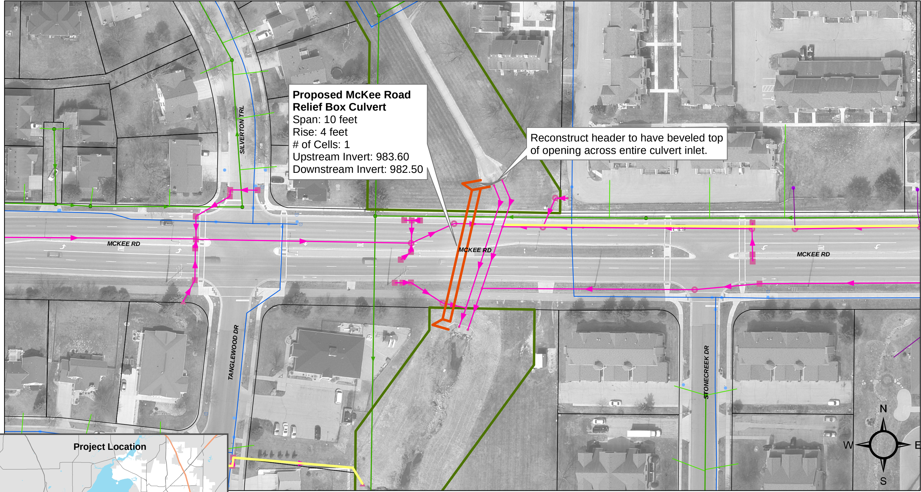
Figure 9-8 McKee Road Relief Box Culvert East Badger Mill Creek Watershed
