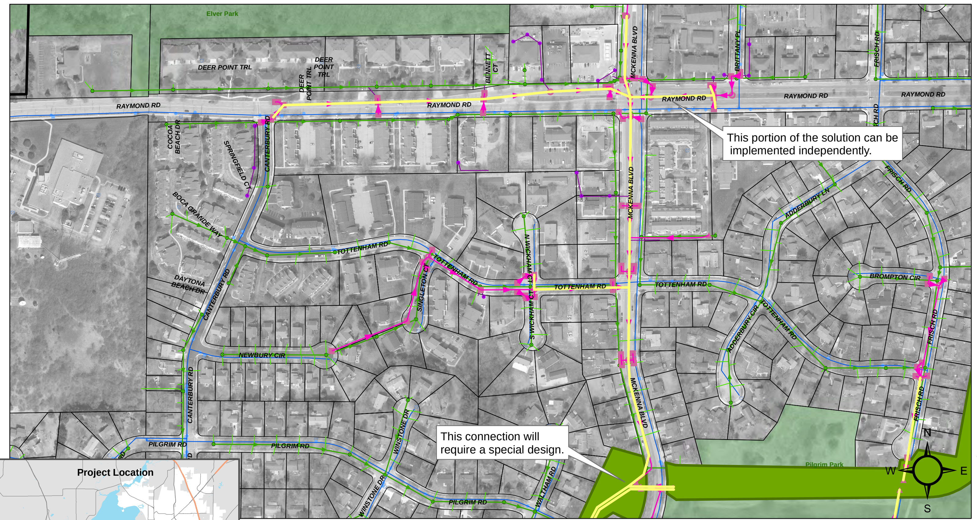
Figure 9-3 McKenna Boulevard- Raymond Road Reconstruction East Badger Mill Creek Watershed
