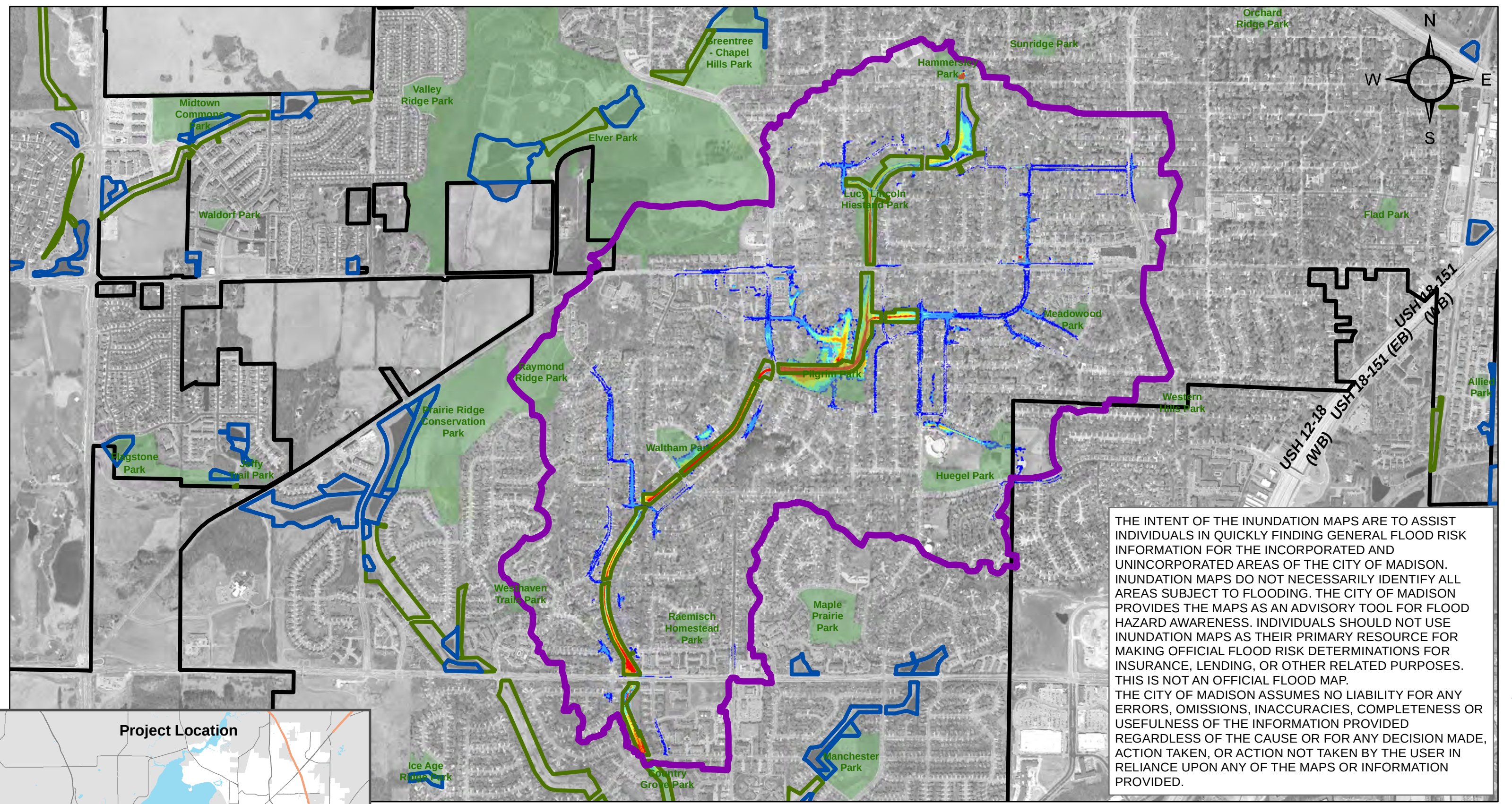
Figure 6-7 Existing Conditions Inundation Mapping 1% Chance Event East Badger Mill Creek Watershed
