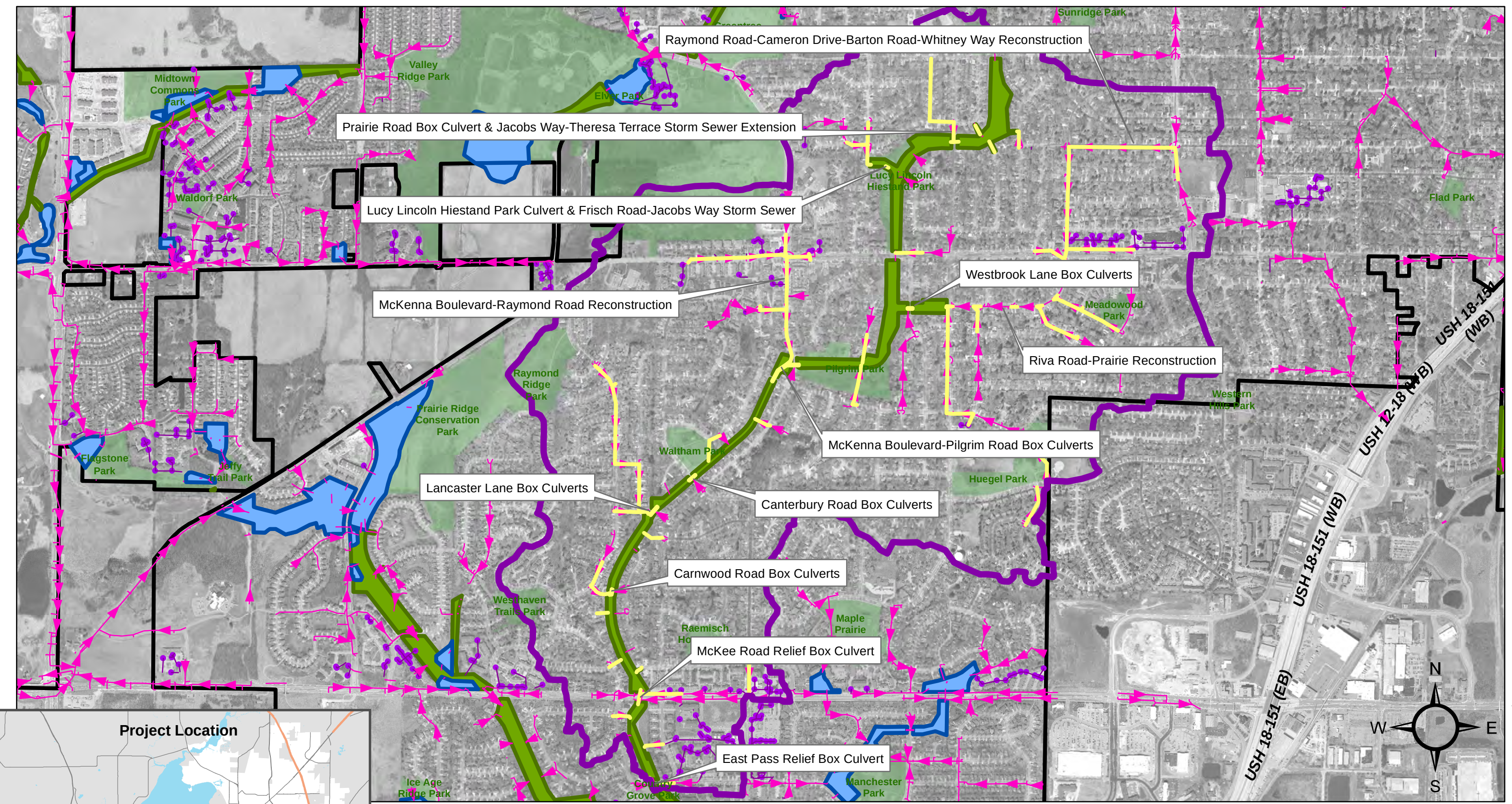
Figure 8-2 Recommended Solutions East Badger Mill Creek Watershed
