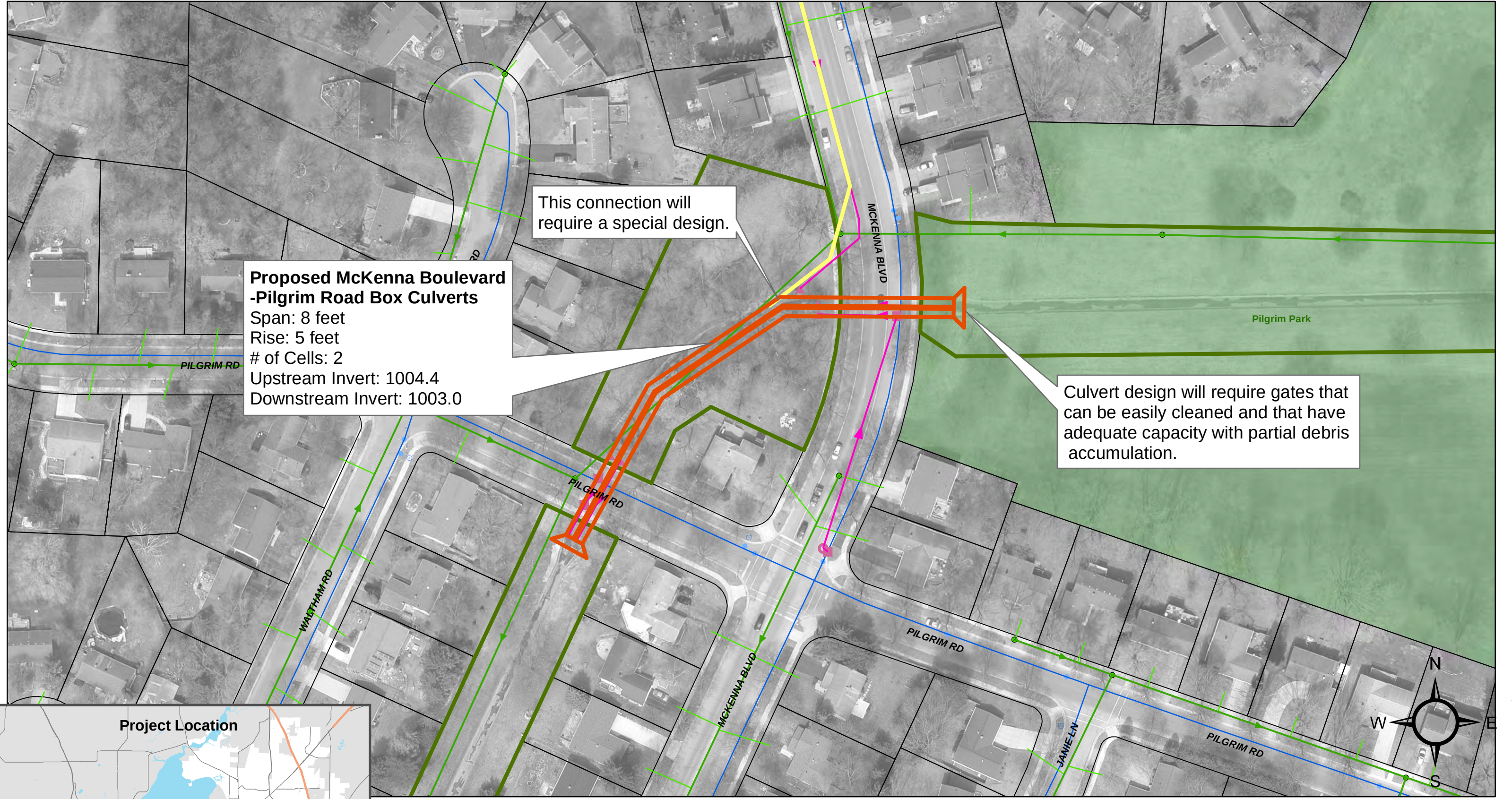
Figure 9-12 McKenna Boulevard-Pilgrim Road Box Culverts East Badger Mill Creek Watershed
