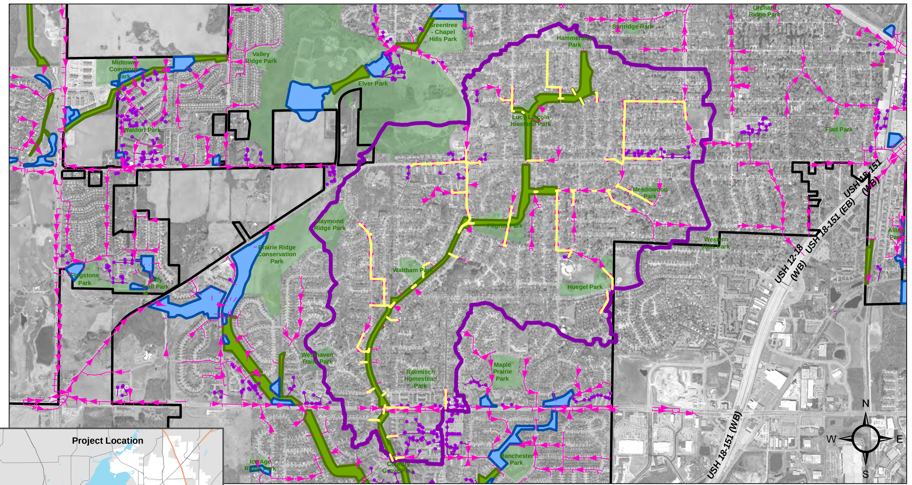
Figure 9-1 Proposed Local Sewer Upgrades East Badger Mill Creek Watershed
