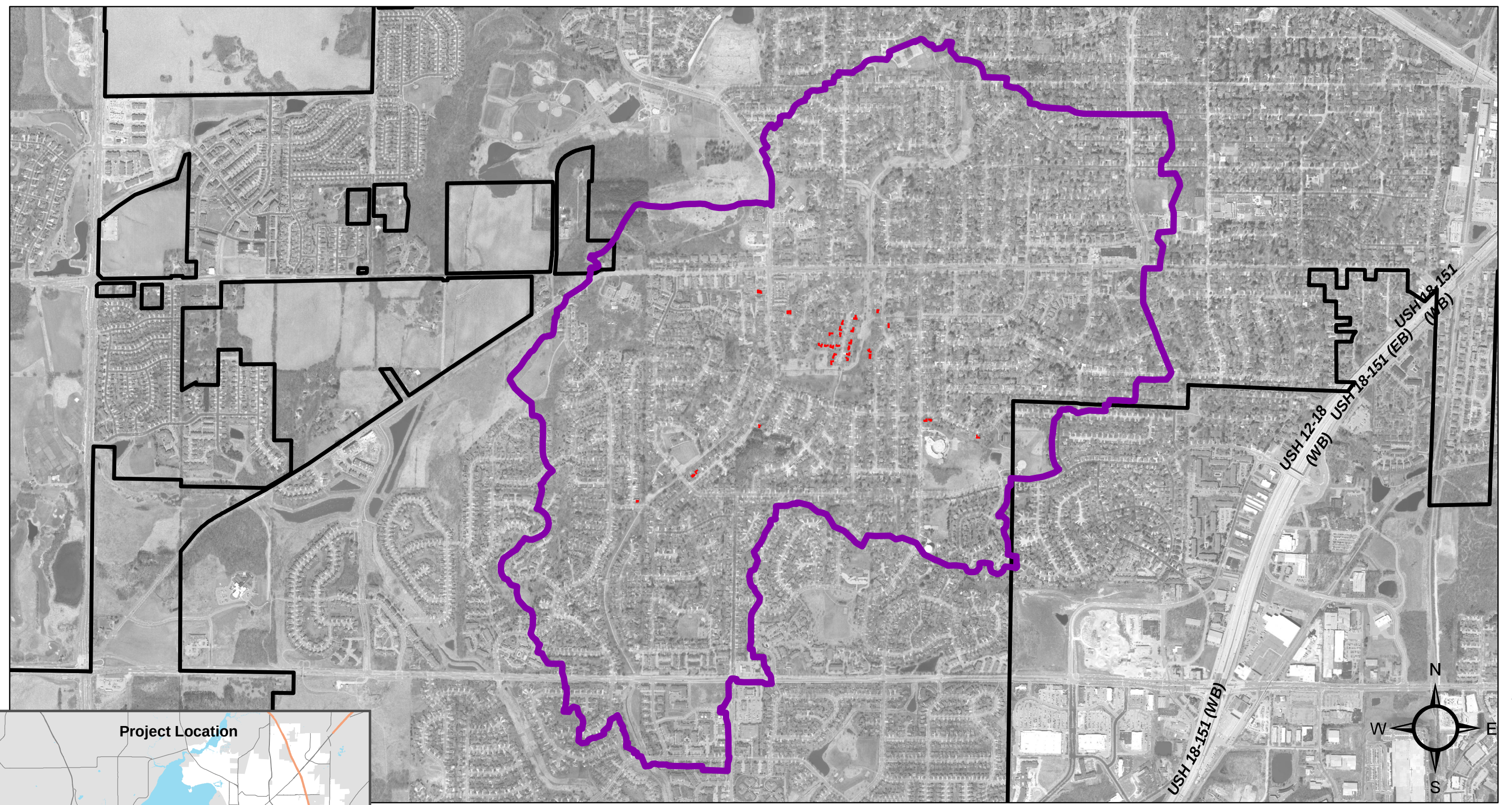
Figure 10-12 Proposed Conditions Structures & Greenway Crossings Not Meeting 1% Chance Event Target East Badger Mill Creek Watershed
