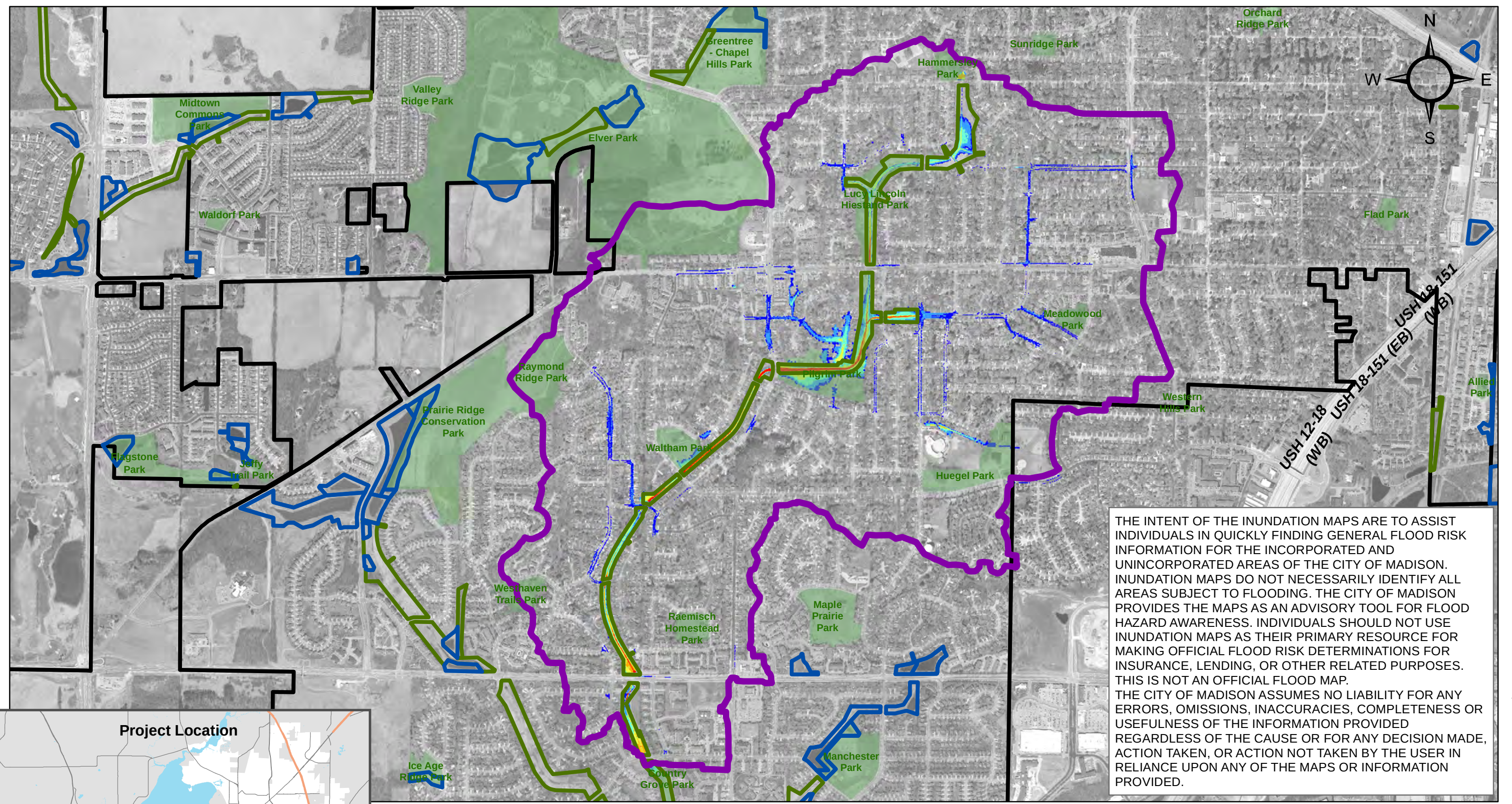
Figure 6-5 Existing Conditions Inundation Mapping 4% Chance Event East Badger Mill Creek Watershed
