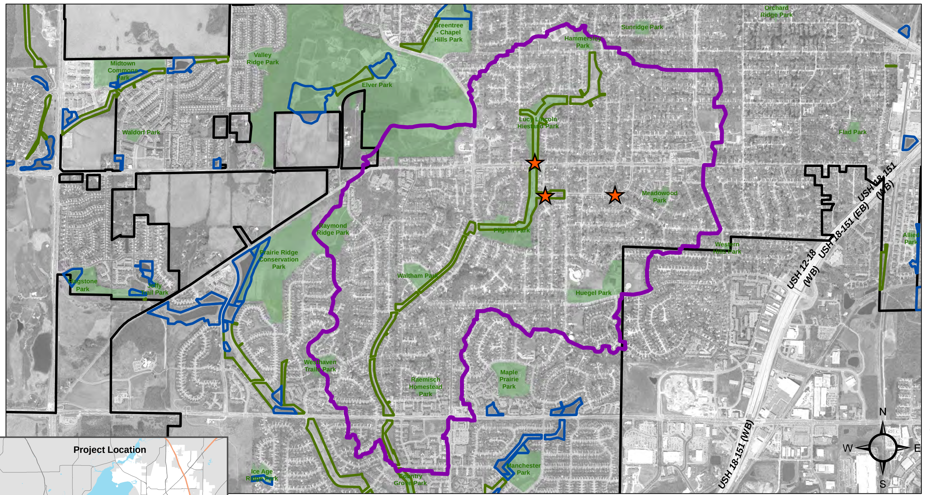
Figure 5-1 Monitoring Locations East Badger Mill Creek Watershed
