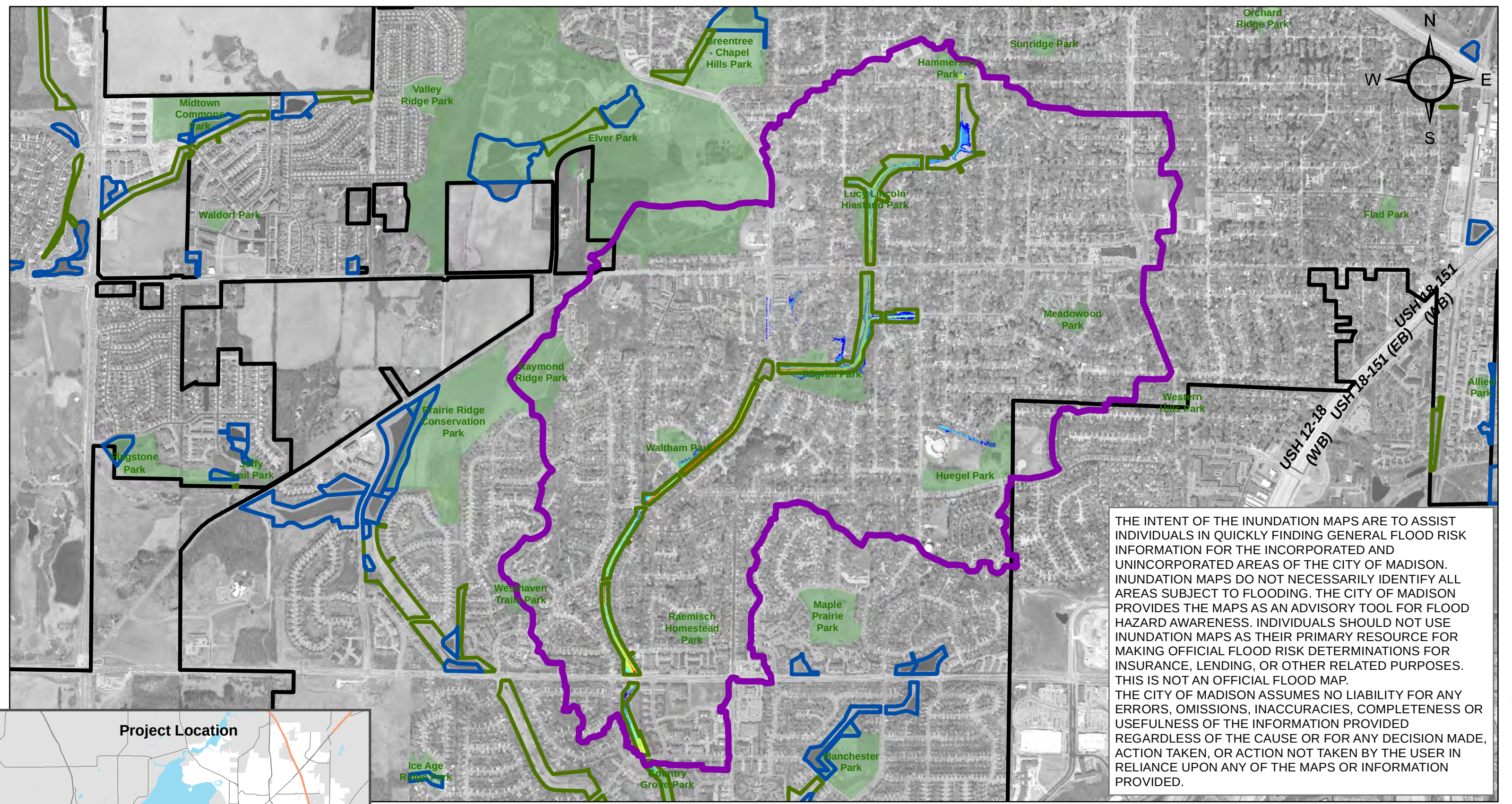
Figure 10-4 Proposed Conditions Inundation Mapping 10% Chance Event East Badger Mill Creek Watershed
