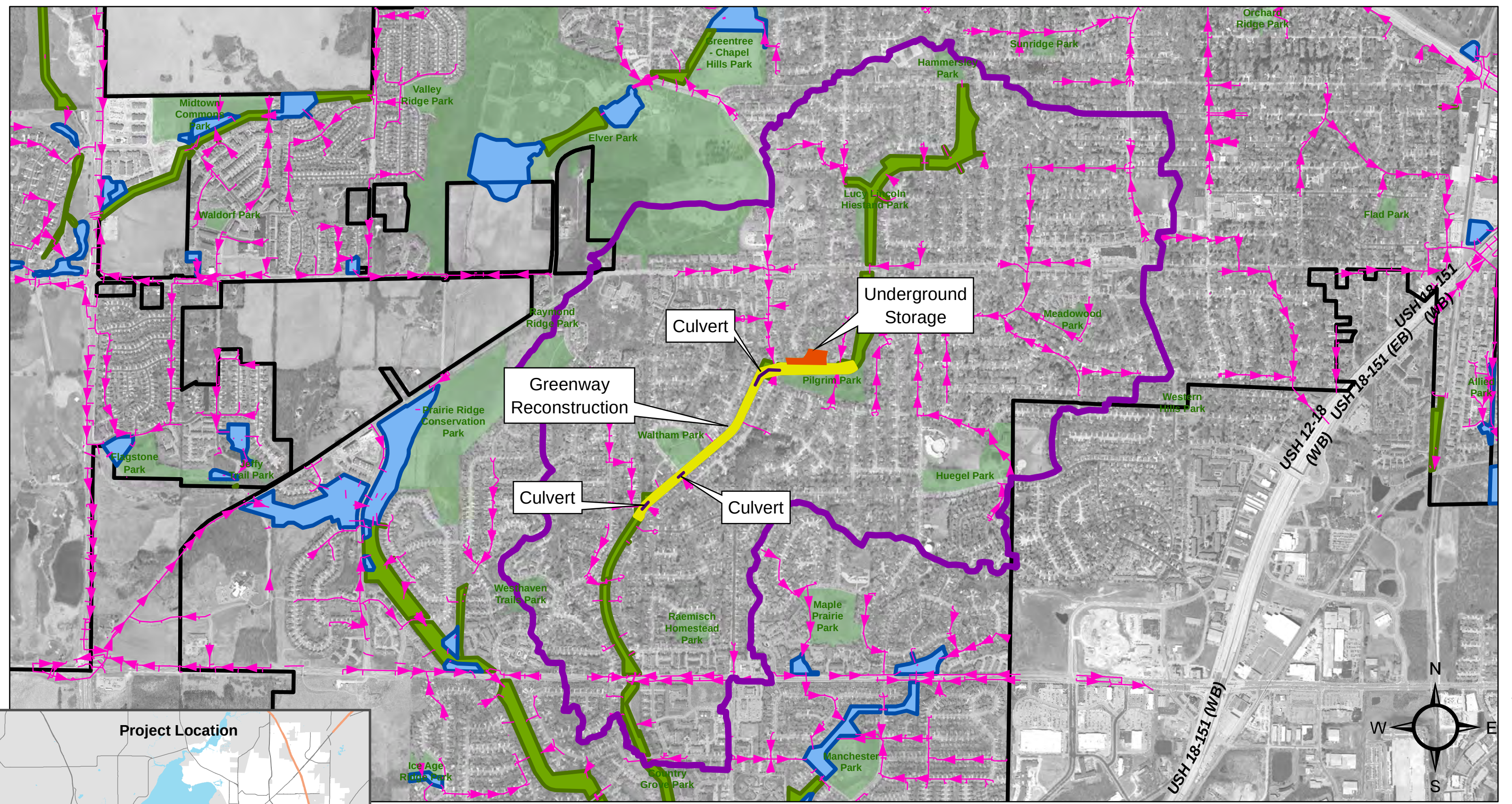
Figure 8-1 Solutions Evaluated - Not Recommended East Badger Mill Creek Watershed
