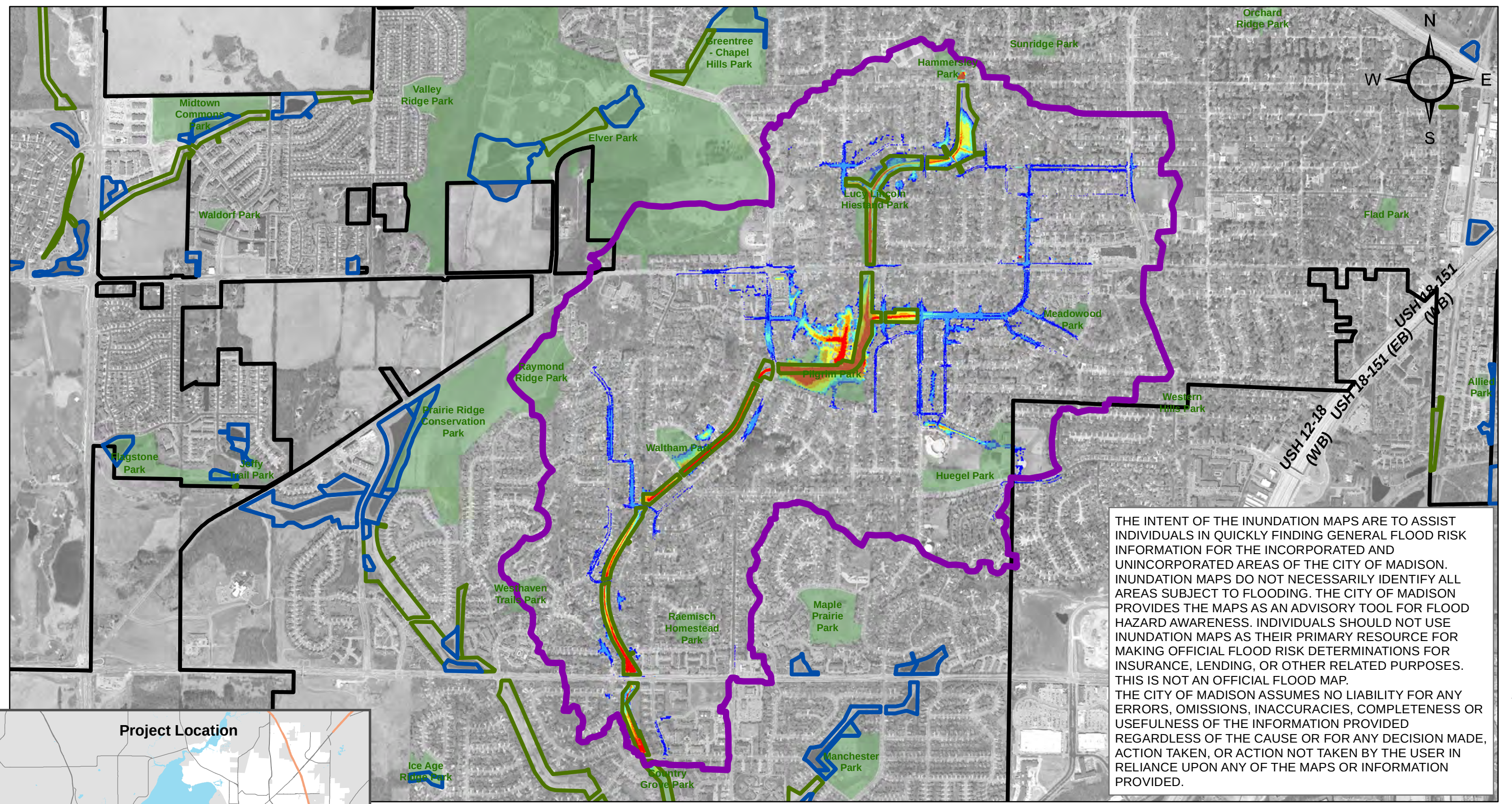
Figure 6-10 Existing Conditions Inundation Mapping August 20th, 2018 Event East Badger Mill Creek Watershed
