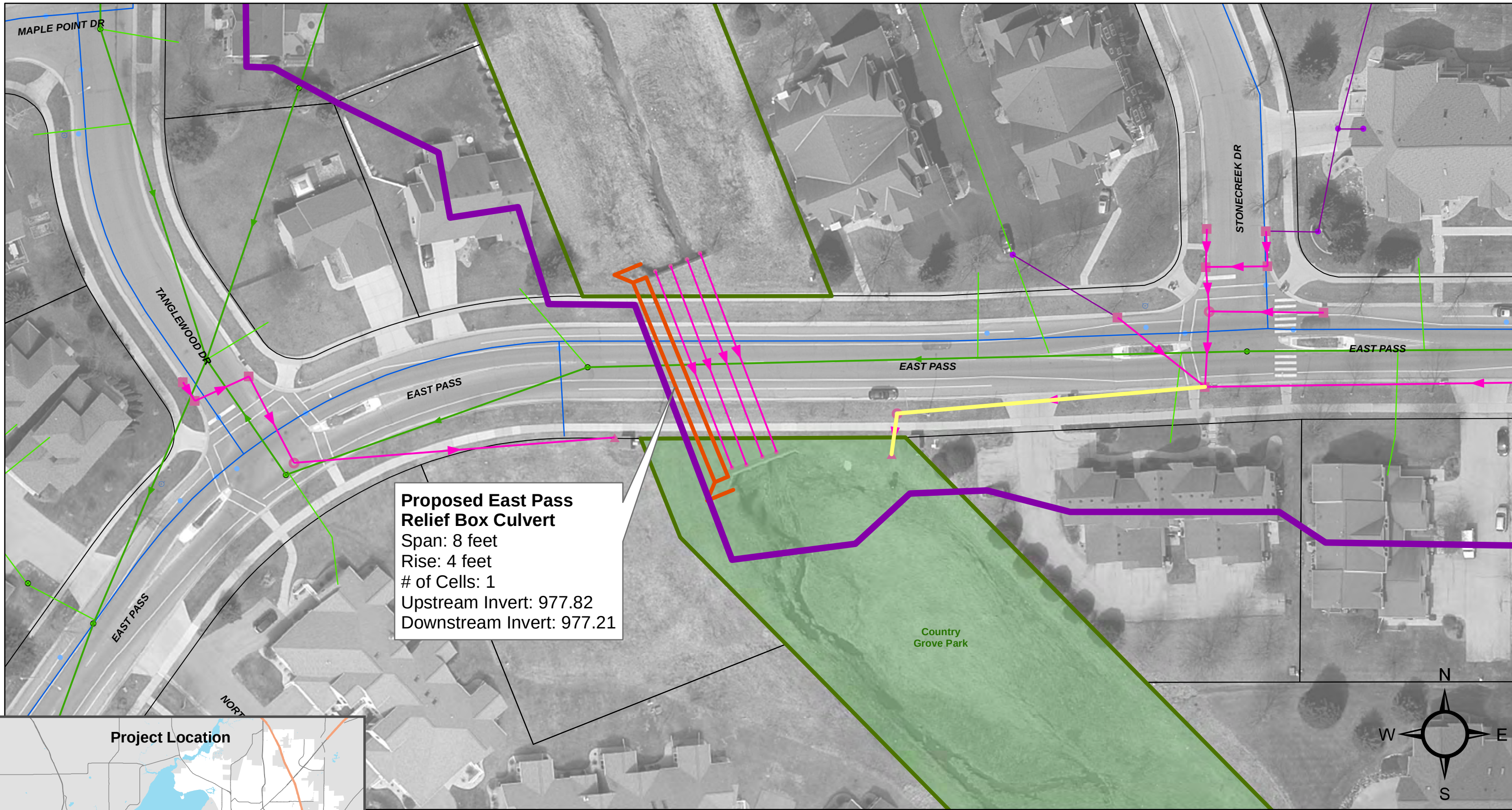
Figure 9-7 East Pass Relief Box Culvert East Badger Mill Creek Watershed
