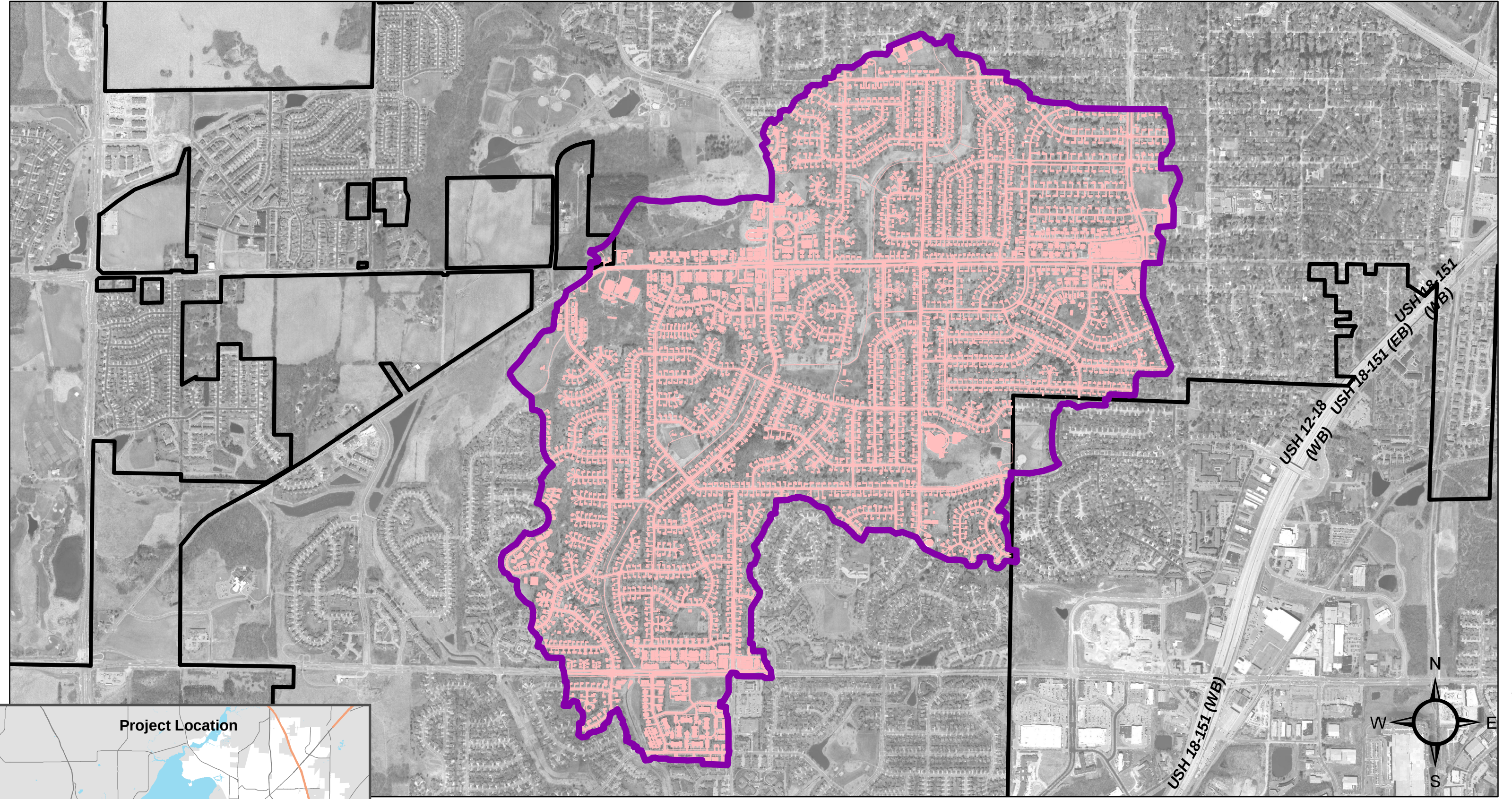
Figure 2-2 Delineated Impervious Areas East Badger Mill Creek Watershed
