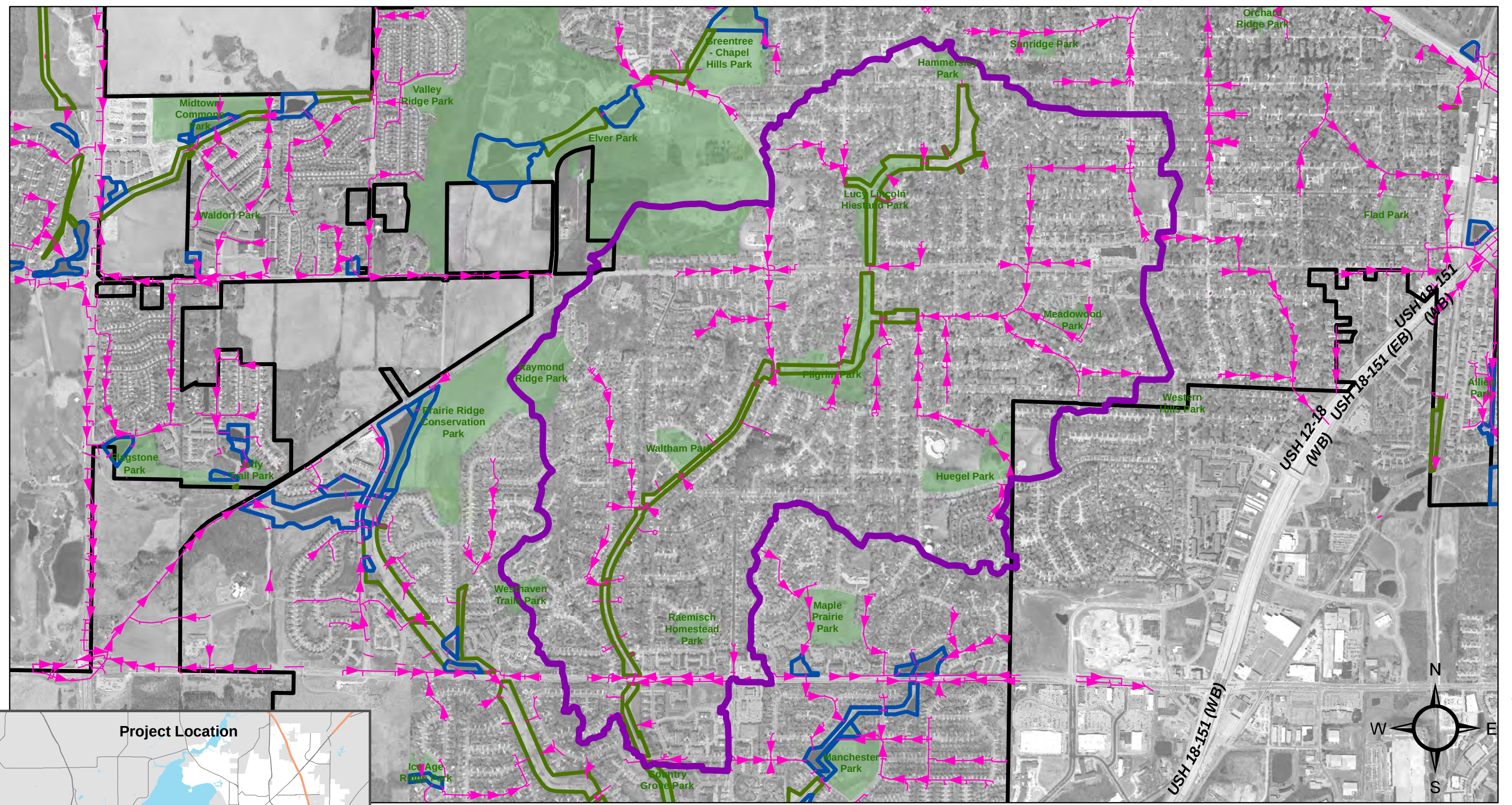
Figure 4-3 Stormwater Conveyance System East Badger Mill Creek Watershed
