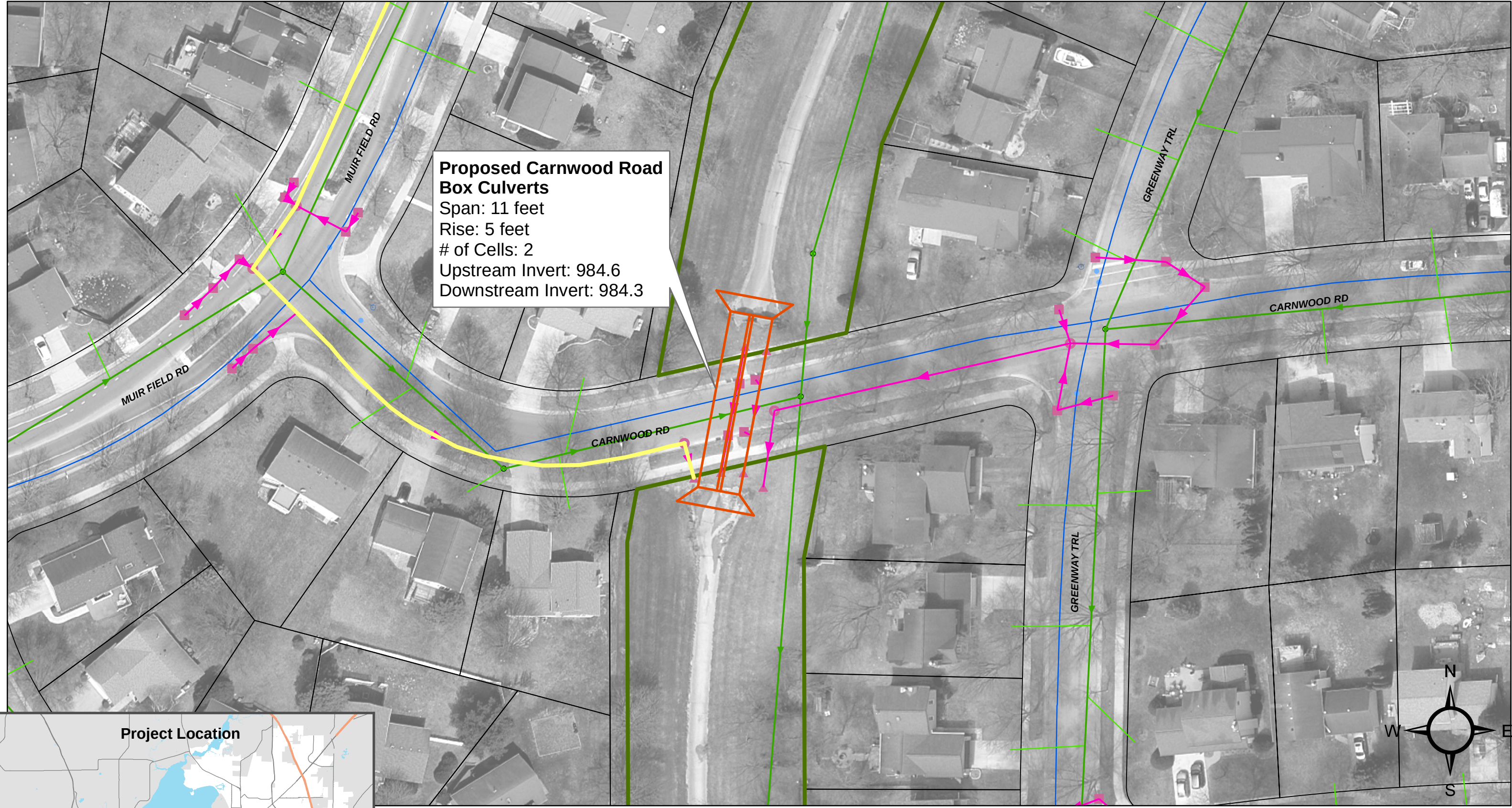
Figure 9-9 Carnwood Road Box Culverts East Badger Mill Creek Watershed
