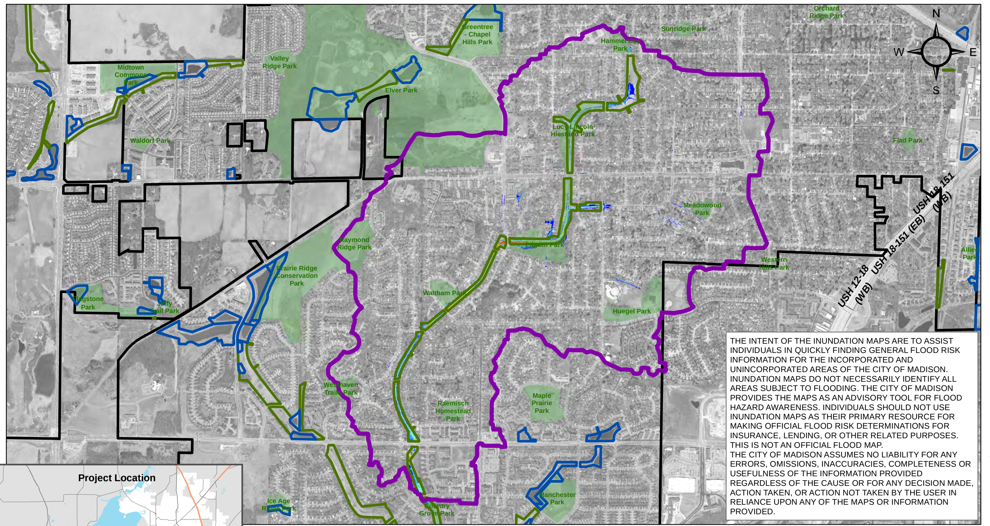
Figure 6-2 Existing Conditions Inundation Mapping 50% Chance Event East Badger Mill Creek Watershed
