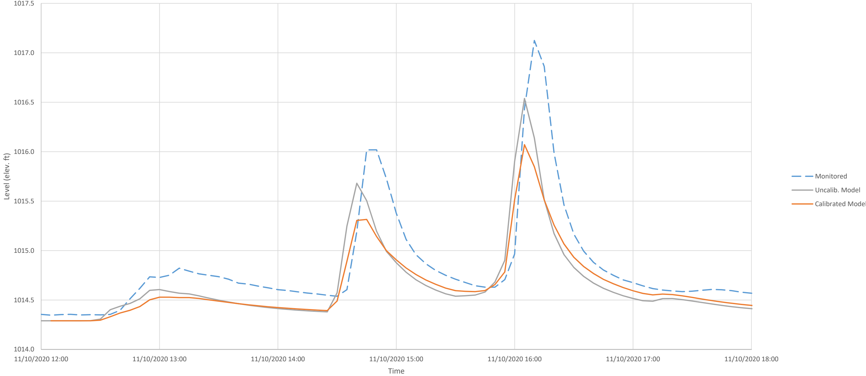
Riva Rd. Level Logger - November 10
